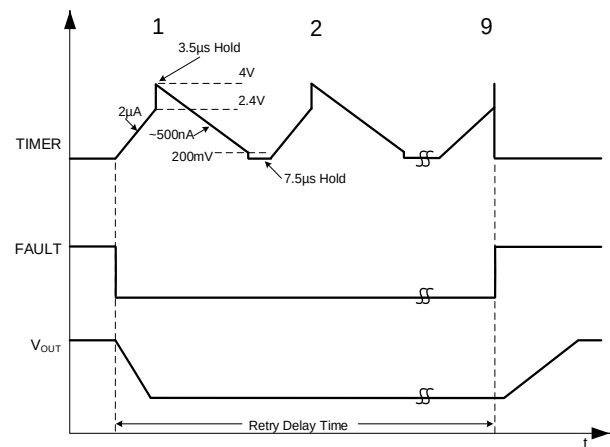
Figure 12: MP5048 Auto-Retry
