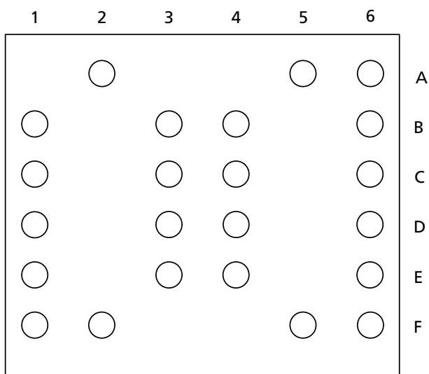
Top view (ball side down)
