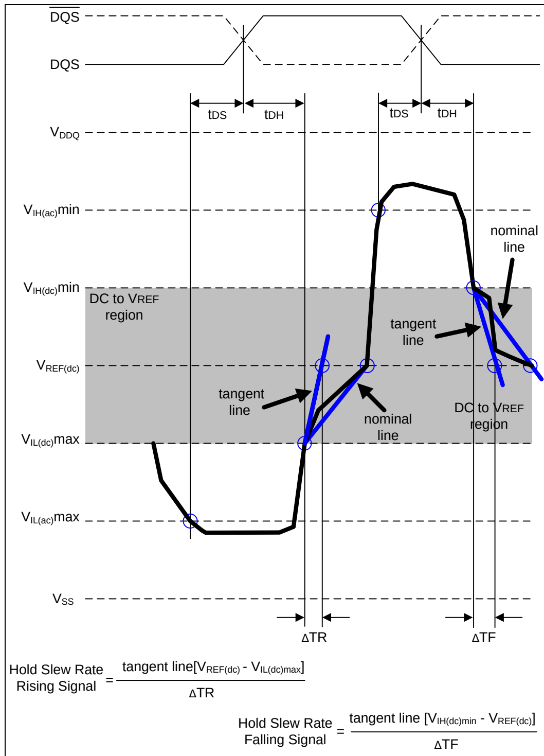
Figure 27 – Illustration tangent line for t_{\text{DH}} (differential \text{DQS}, \overline{\text{DQS}} )
