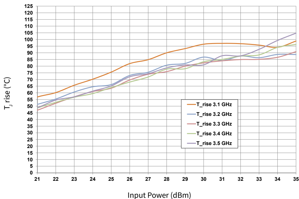
Figure 5. CGHV35060MP-AMP1 T_j rise vs. Input Power V_{DD} = 50\text{ V} I_{DQ} = 125\text{ mA} , Pulse Width = 100\mu\text{s} , Duty Cycle = 10%, T_{CASE} = 25^\circ\text{C}
