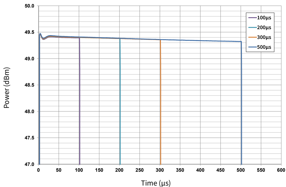
Figure 6. CGHV35060MP-AMP1 Output Power vs. Time, Varying Pulse Lengths V_{DD} = 50\text{ V} P_{IN} = 35\text{ dBm} , Duty Cycle = 10%
