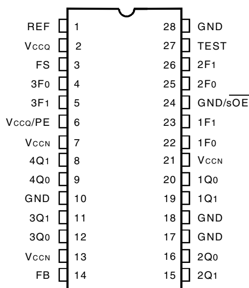
QSOPTOP TOP VIEW
