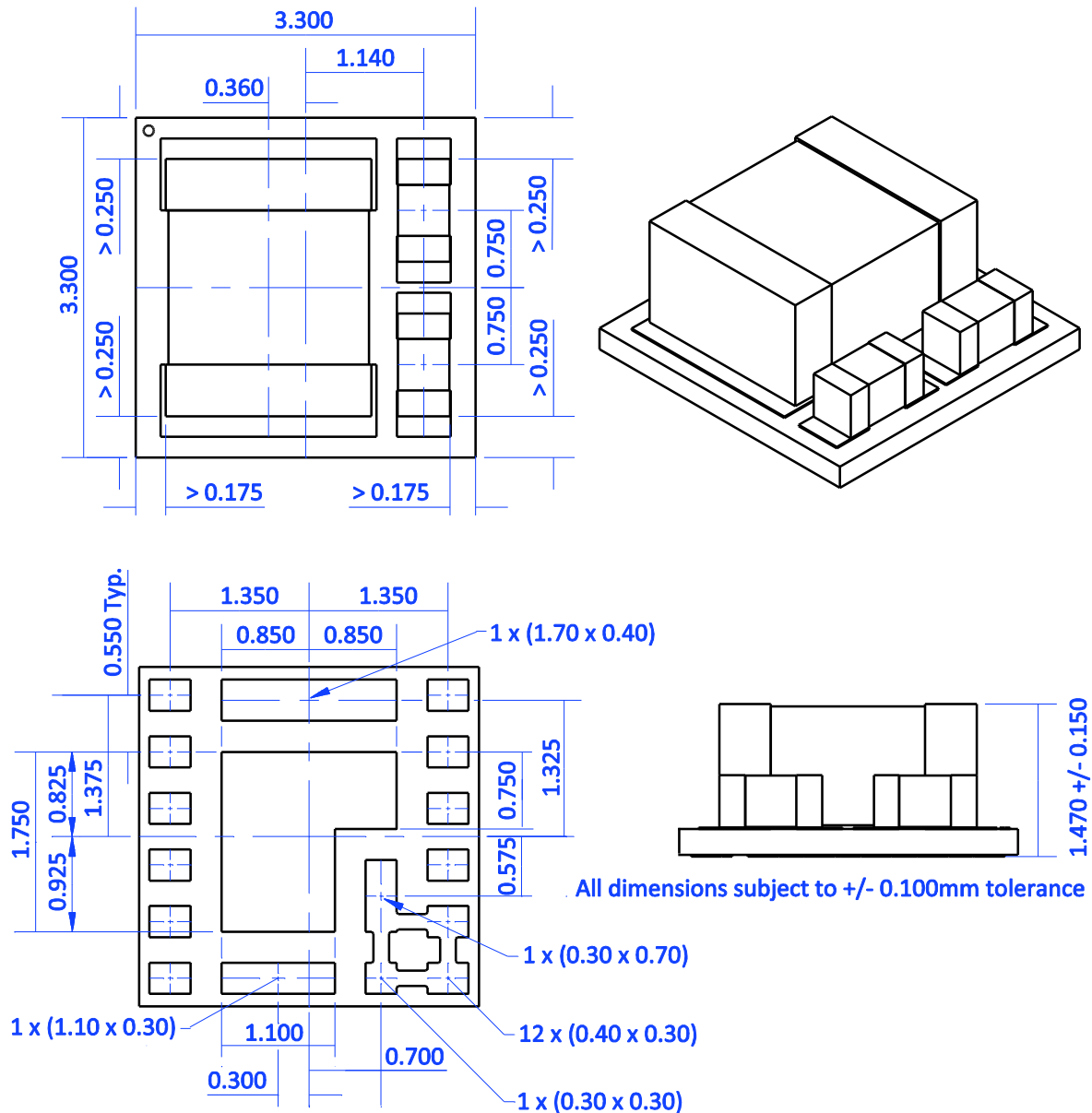
Figure 30 Dimensioned drawings
