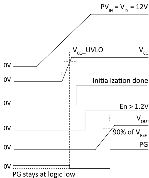
Figure 10 Start-up: En pin asserted after PV IN and V IN , PG pin pulled up to an external supply
