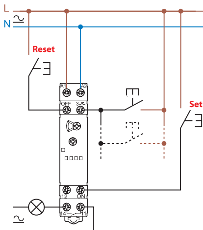
Type 13.61.8.230 - Examples of multiple 4 wire connection with centralized reset push-button
