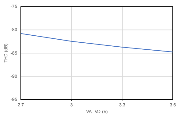
Figure 17. THD vs. power supply
