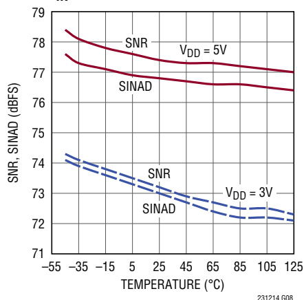
SNR, SINAD vs Temperature, f_{IN} = 259\text{kHz}
