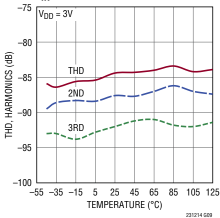
THD, Harmonics vs Temperature, f_{IN} = 259\text{kHz}
