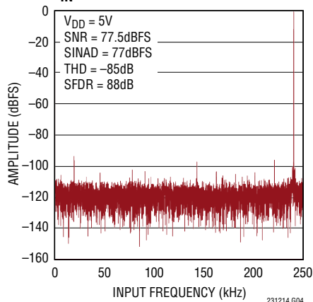
16k Point FFT, f_S = 500\text{ksps} , f_{IN} = 259\text{kHz}
