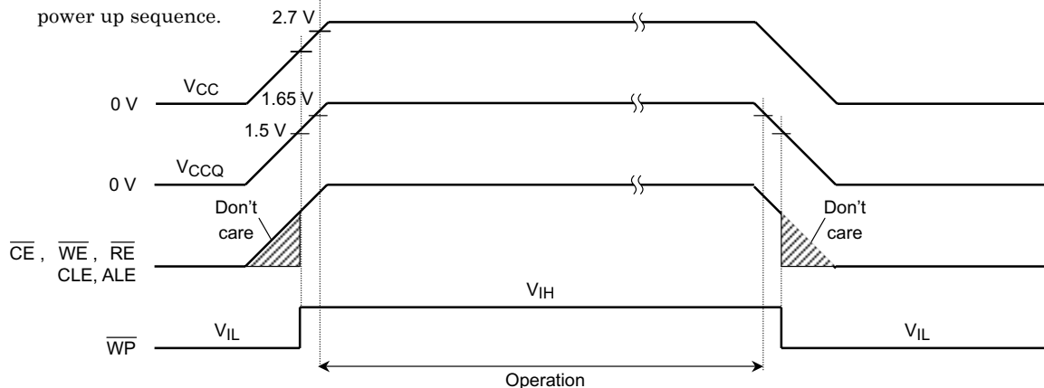
Figure 15. Power-on/off Sequence
