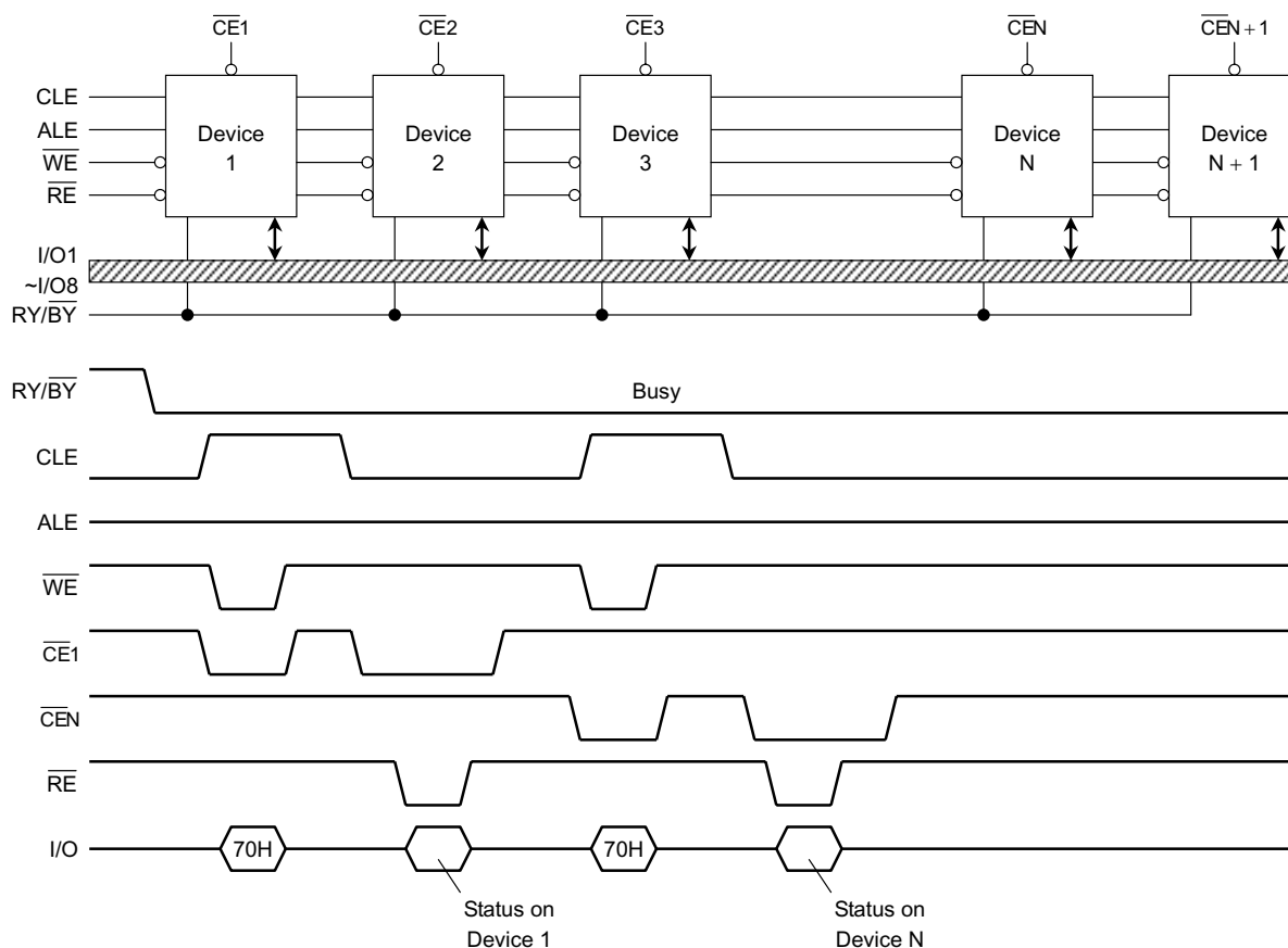
Figure 6. Status Read timing application example
