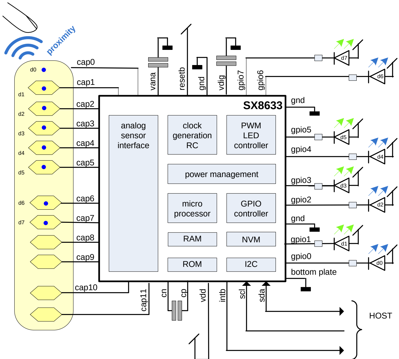
Figure 50 Typical Application
