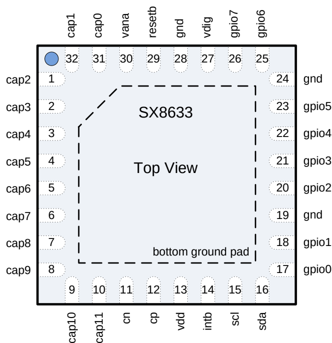
Figure 1 Pinout Diagram
