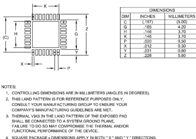
Figure 59 Land Pattern
