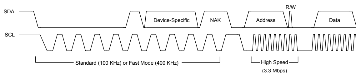
Figure 21-7. High-Speed Data Format
