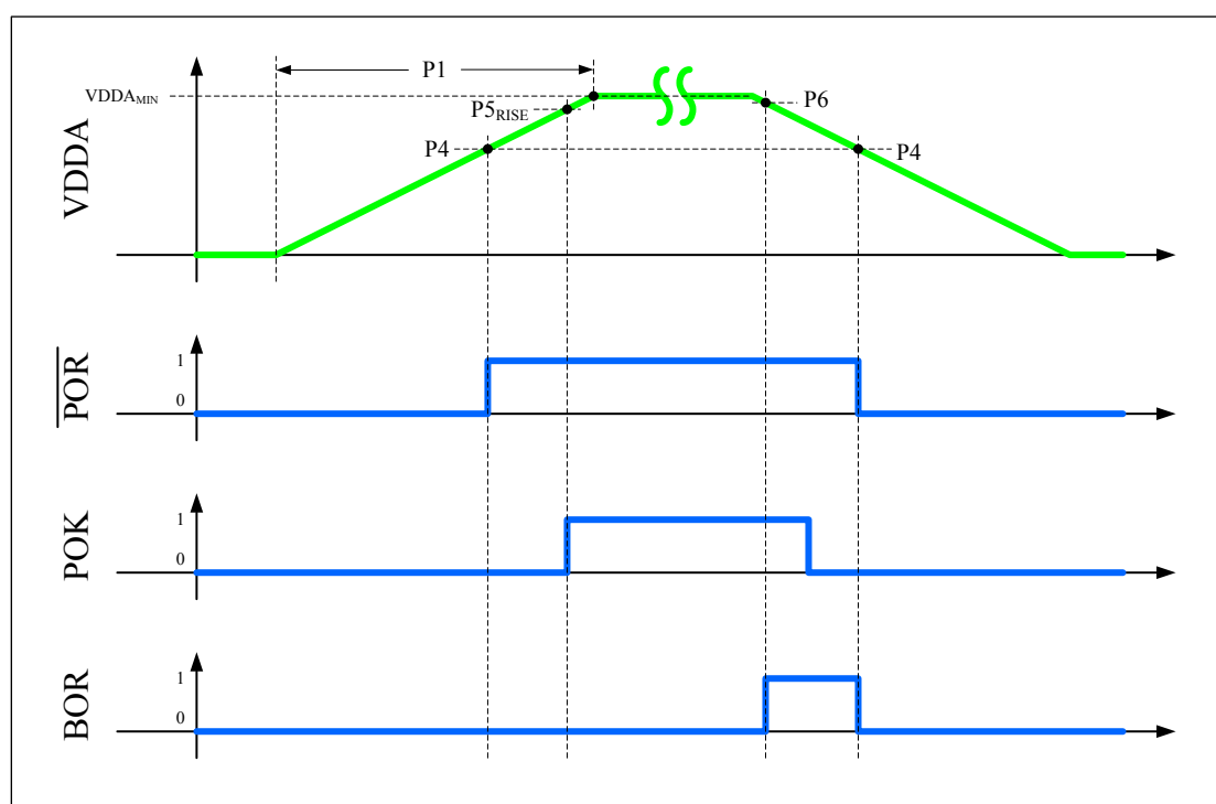
Figure 32-4. Power and Brown-Out Assertions vs V_{DDA} Levels
