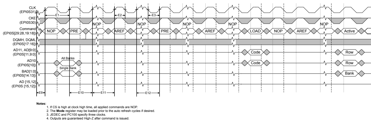
Figure 32-18. SDRAM Initialization and Load Mode Register Timing
