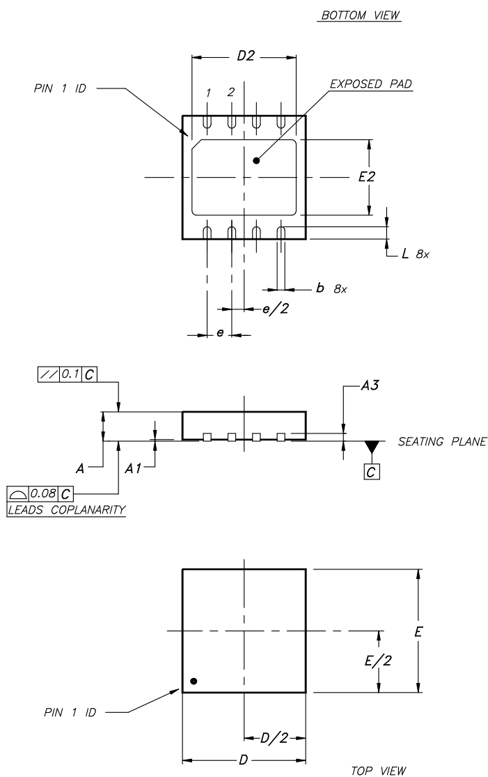
Figure 32. VFQFPN8 (4x4x1.08 mm) package outline
