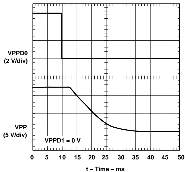
Figure 13. VPP Propagation Delay and Fall Time With 150-μF Load, 12-V Switch
