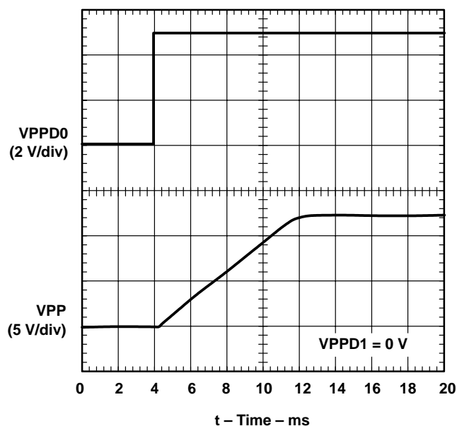
Figure 12. VPP Propagation Delay and Rise Time With 150-μF Load, 12-V Switch
