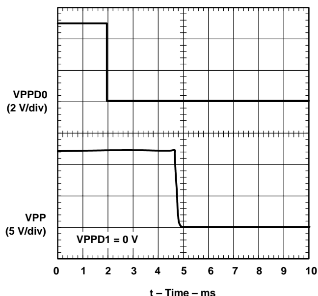
Figure 11. VPP Propagation Delay and Fall Time With 1-μF Load, 12-V Switch
