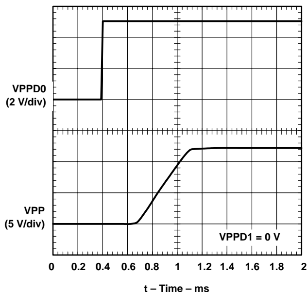
Figure 10. VPP Propagation Delay and Rise Time With 1-μF Load, 12-V Switch
