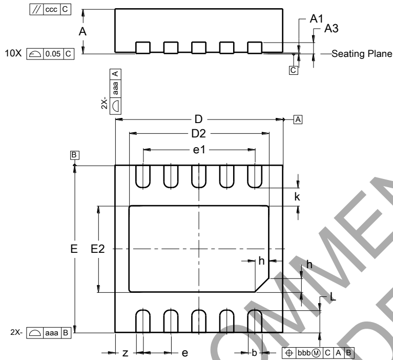
V-DFN3030-10 (Standard)
