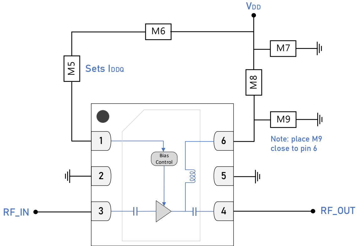
GRF2501 Standard Evaluation Board Schematic
