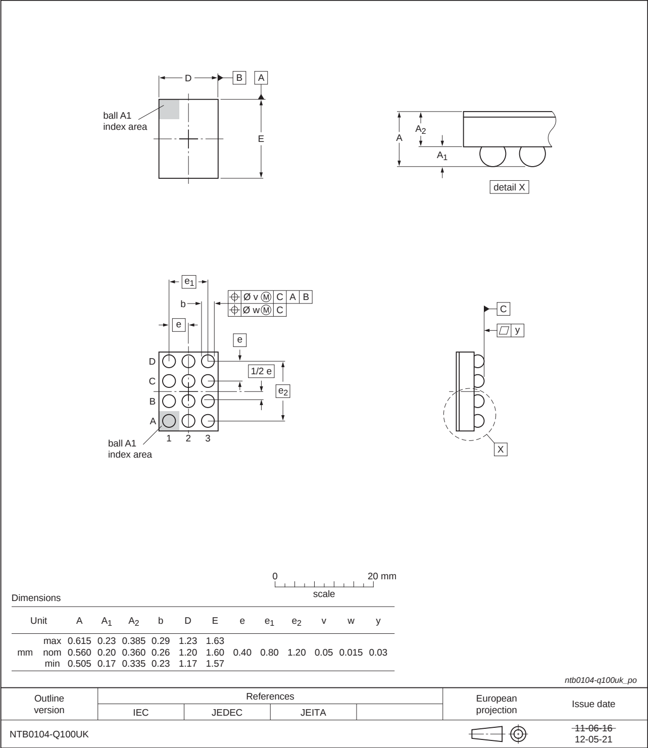
Fig 10. Package outline WLCSP12 package
