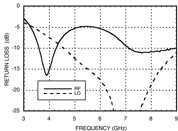
Return Loss
