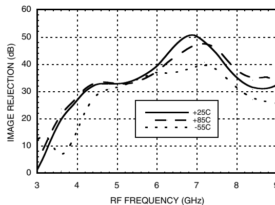
Image Rejection vs. Temperature
