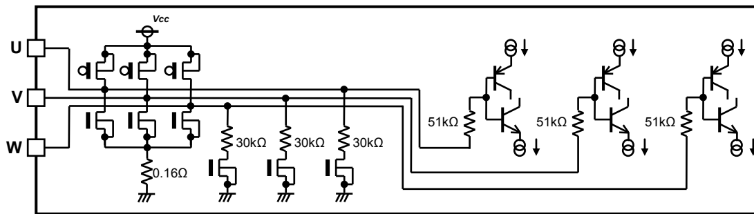
Figure 30. I/O equivalent circuits
