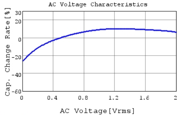
GRM155C80J105KE15 C-AC Voltage capchange, Dc
