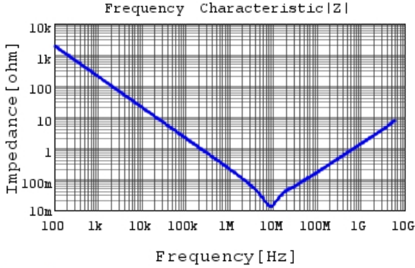
GRM155C80J105KE15 |Z| DCOV, 25degC
