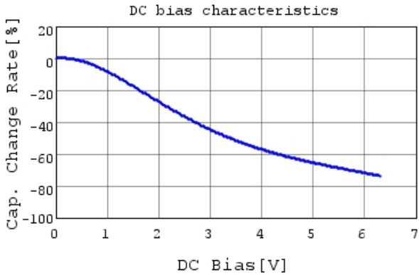
GRM155C80J105KE15 C-DC bias capchange, 25.0c
