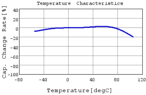
GRM155C80J105KE15 C-Temp. capchange, DC0.0V,
