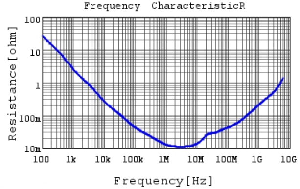
GRM155C80J105KE15 R DCOV, 25degC
