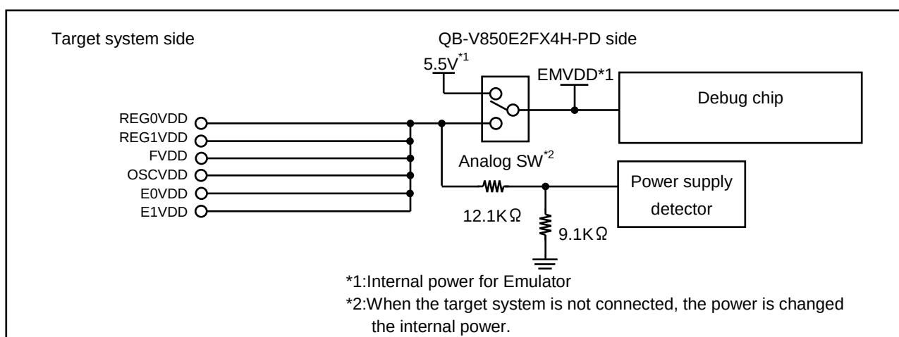
Figure A-2. Equivalent Circuit B
