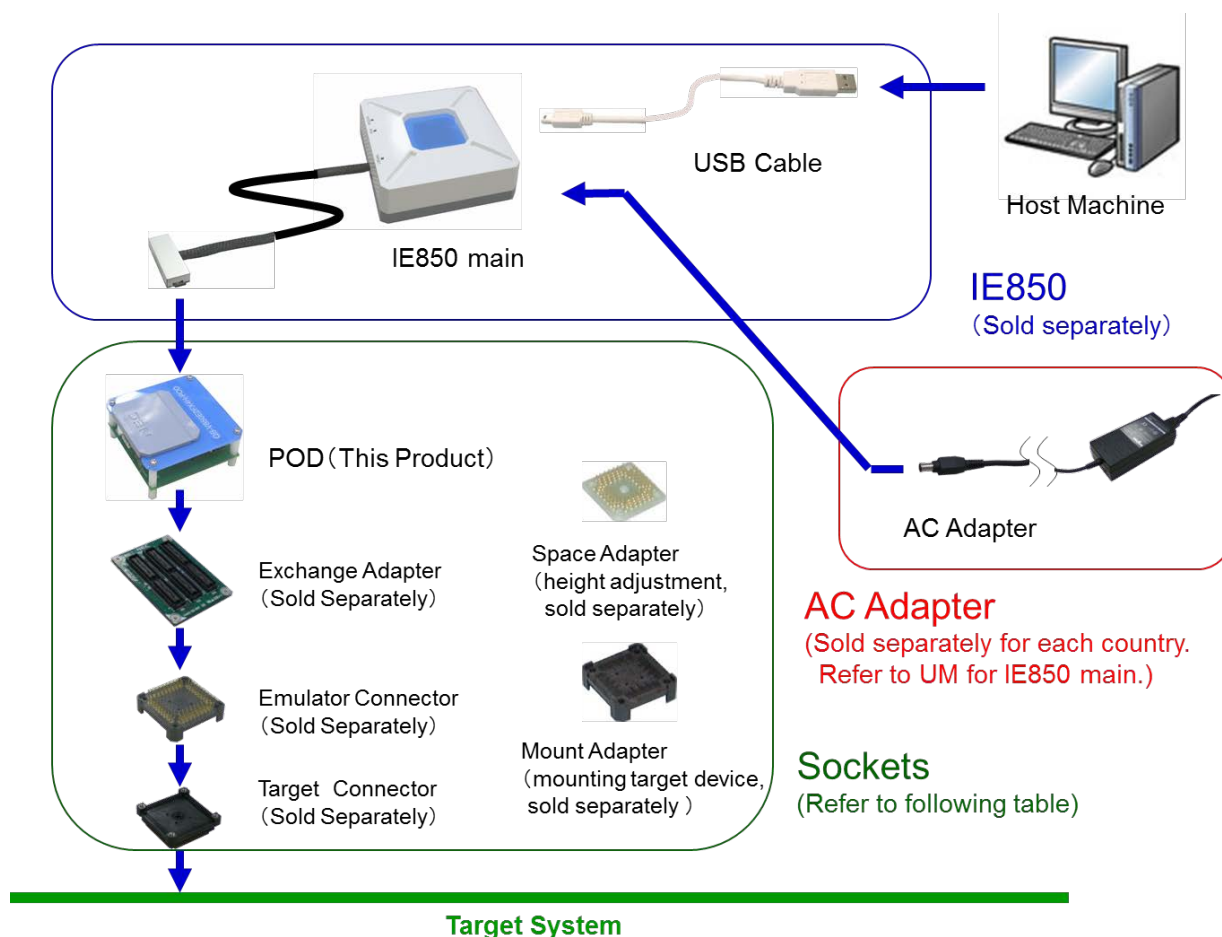
Figure 1-2. System Configuration
