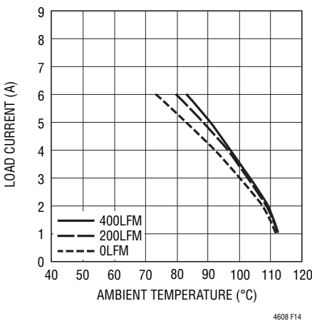
Figure 14. BGA Heat Sink with 3.3V IN to 2.5V OUT
