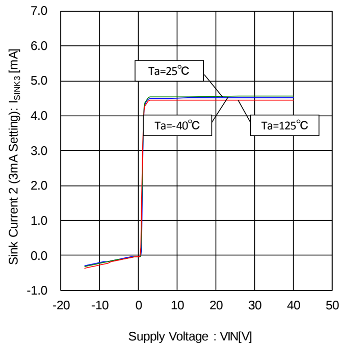
Figure 46. Sink Current 2- Voltage Characteristic (3mA Setting)
