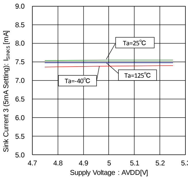
Figure 52. Sink Current 3- Voltage Characteristic (5mA Setting, 8V external supply)
