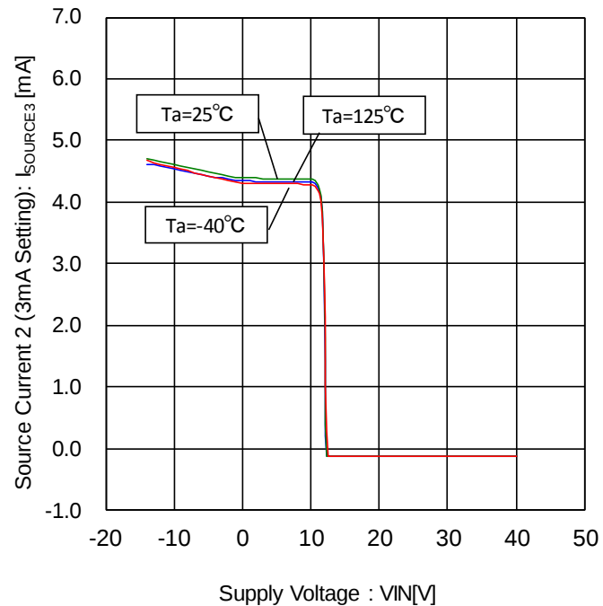
Figure 42. Source Current 2- Voltage Characteristic (3mA Setting)
