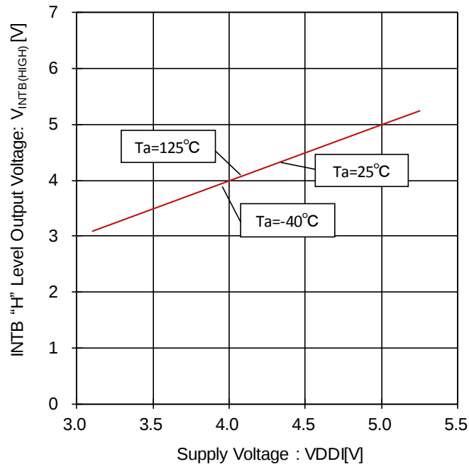
Figure 102. INTB “H” Level Output Voltage- Voltage Characteristic (INTB=OPEN)
