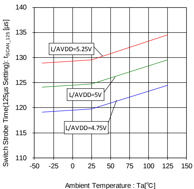
Figure 111. Switch Strobe Time- Temperature Characteristic (125µs Setting)
