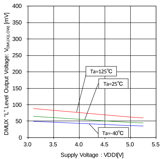
Figure 98. DMUX "L" Level Output Voltage- Voltage Characteristic ( I_{SINK}=1.6mA )
