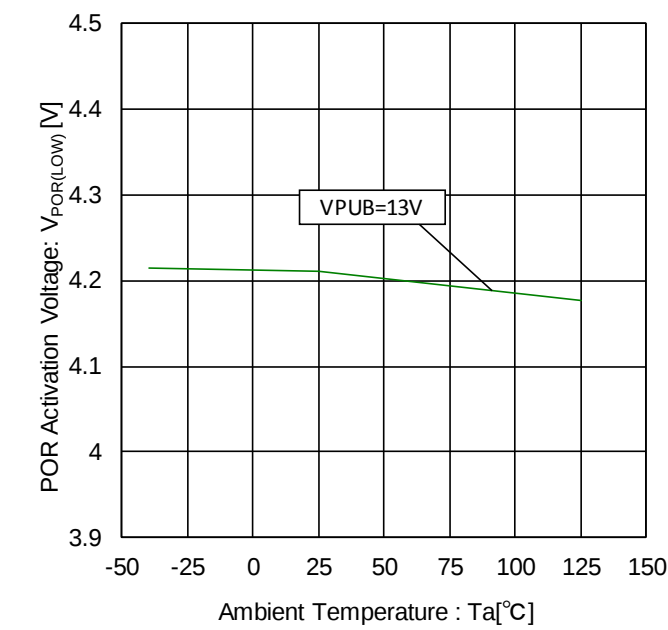
Figure 21. POR (Power on Reset) Activation Voltage - Temperature Characteristic
