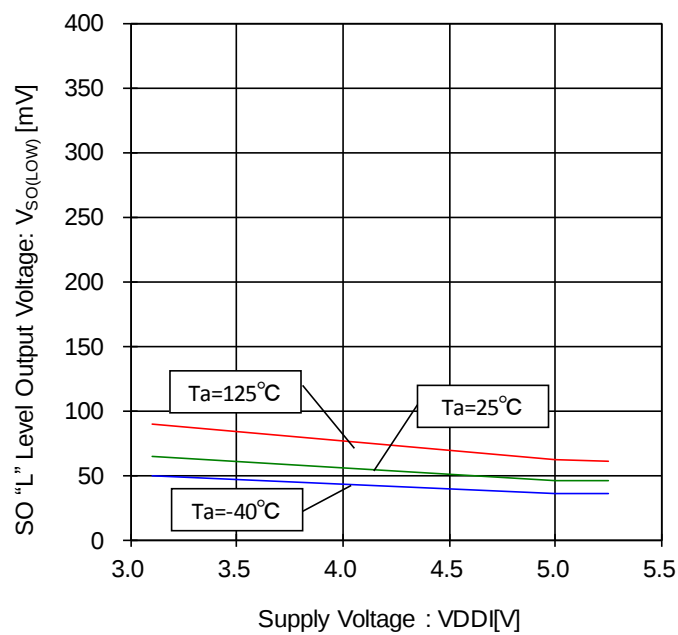
Figure 92. SO "L" Level Output Voltage- Voltage Characteristic ( I_{SINK}=1.6mA )
