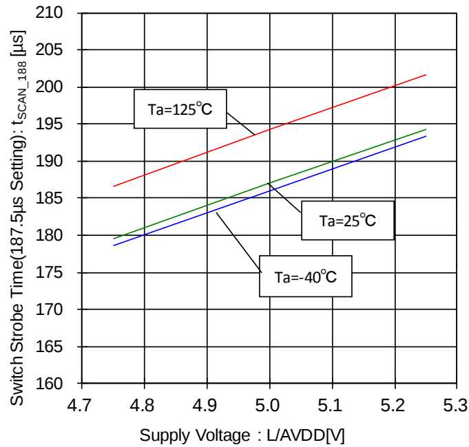
Figure 114. Switch Strobe Time- Voltage Characteristic (187.5µsSetting)
