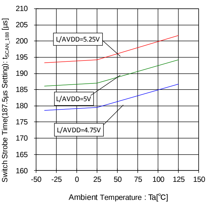
Figure 113. Switch Strobe Time- Temperature Characteristic (187.5µsSetting)
