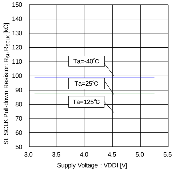
Figure 86. SI, SCLK Pull-down Resistor- Voltage Characteristic
