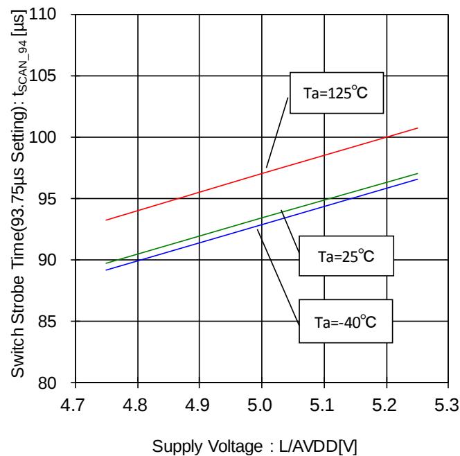
Figure 110. Switch Strobe Time- Voltage Characteristic (93.75µs Setting)
