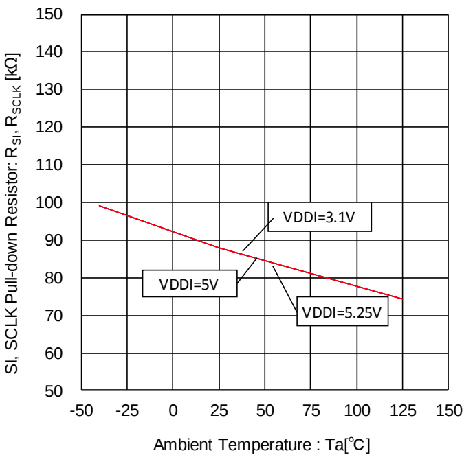
Figure 85. SI, SCLK Pull-down Resistor- Temperature Characteristic
