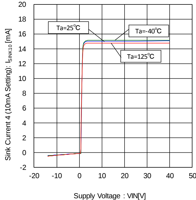
Figure 62. Sink Current 4- Voltage Characteristic (10mA Setting)
