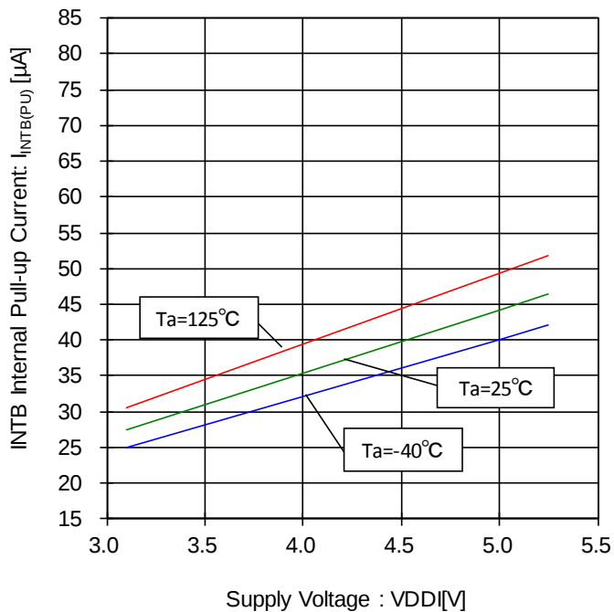
Figure 100. INTB Internal Pull-up Current- Voltage Characteristic
