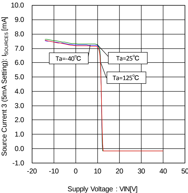
Figure 50. Source Current 3- Voltage Characteristic (5mA Setting)
