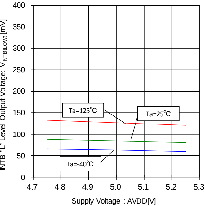
Figure 104. INTB “L” Level Output Voltage- Voltage Characteristic ( I_{SINK}=1.0mA )
