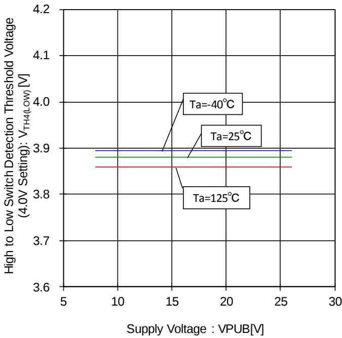
Figure 78. High to Low Switch Detection Threshold Voltage - Voltage Characteristic (4.0V Setting)
