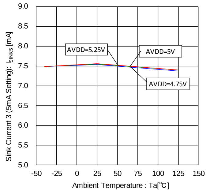
Figure 51. Sink Current 3- Temperature Characteristic (5mA Setting, 8V external supply)
