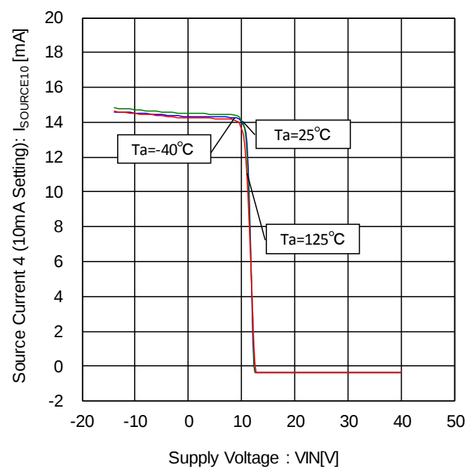
Figure 58. Source Current 4- Voltage Characteristic (10mA Setting)
