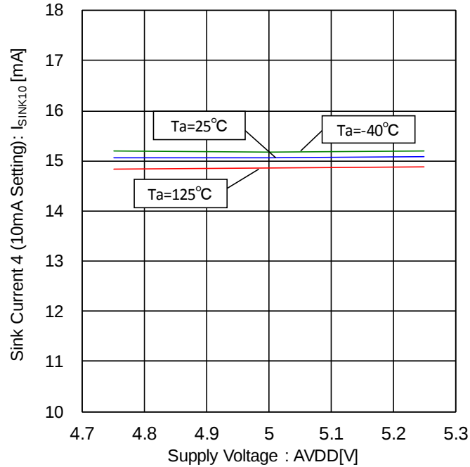
Figure 60. Sink Current 4- Voltage Characteristic (10mA Setting, 8V external supply)
