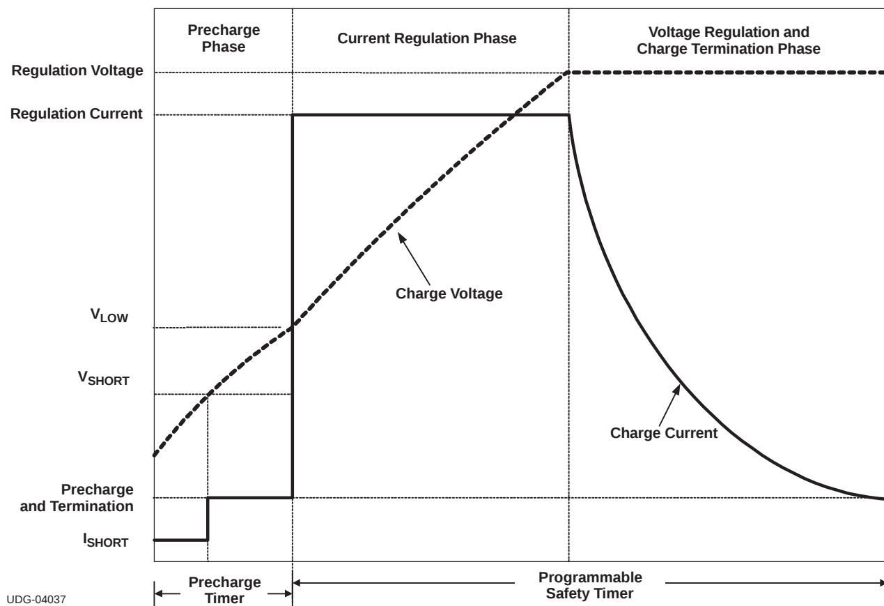
Figure 3. Typical Charging Profile
