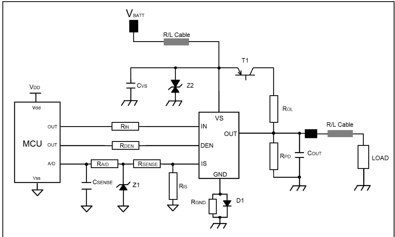
Figure 37. Application Diagram
