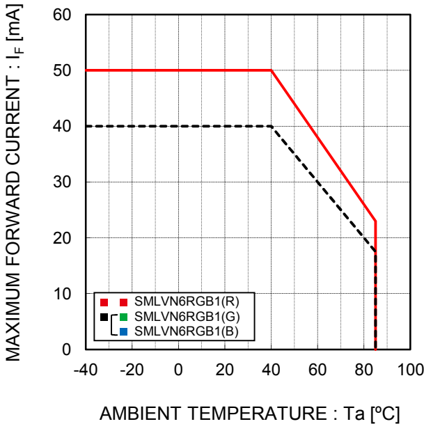
Fig.5 Derating
