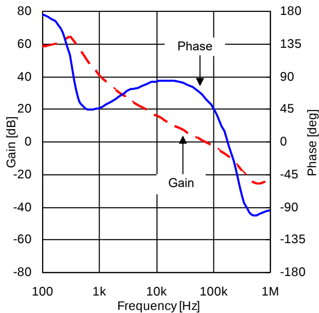
Figure 52. Frequency Characteristic ( V_{IN} = 12\text{ V} , I_{OUT} = 1.0\text{ A} )
