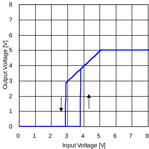
Figure 84. Output Voltage vs Input Voltage 1 ( R_{LOAD} = 250 \Omega )
