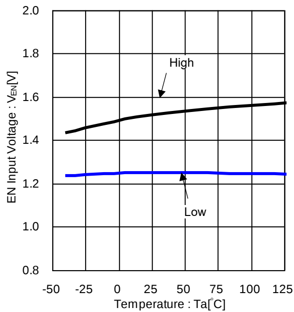
Figure 15. EN Input Voltage vs Temperature
