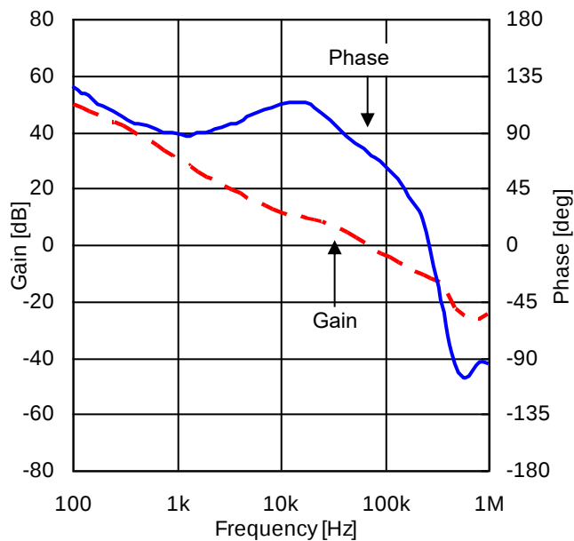
Figure 78. Frequency Characteristic ( V_{IN} = 12\text{ V} , I_{OUT} = 1.0\text{ A} )
