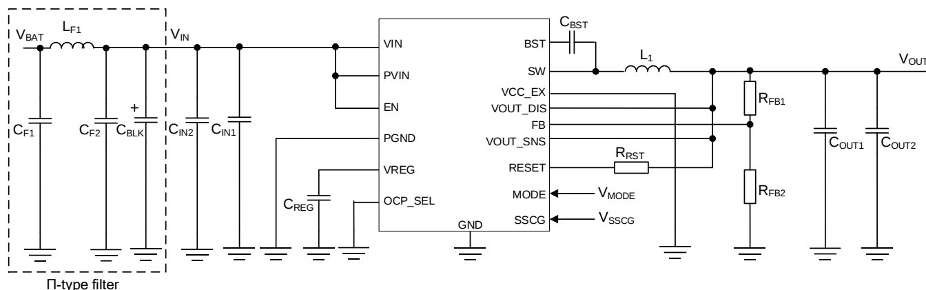
Figure 49. Reference Circuit 1
