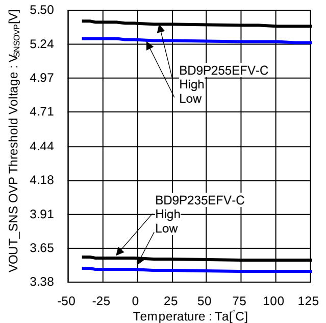
Figure 28. VOUT_SNS OVP Threshold Voltage vs Temperature (BD9P235EFV-C/BD9P255EFV-C)
