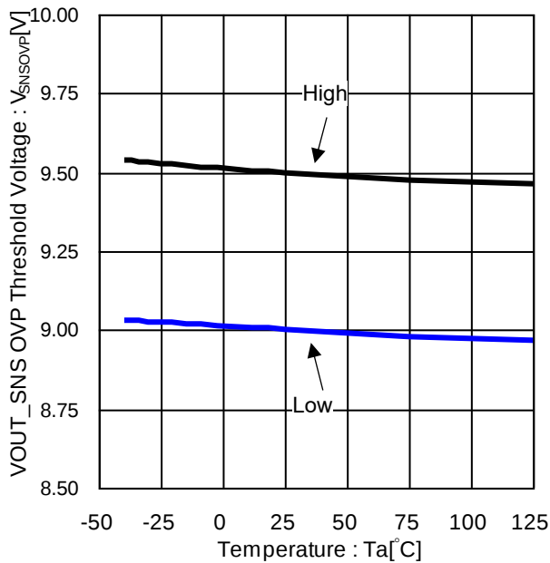
Figure 27. VOUT_SNS OVP Threshold Voltage vs Temperature (BD9P205EFV-C)
