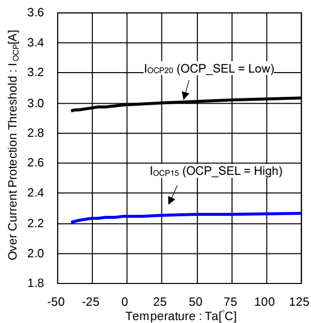
Figure 20. Over Current Protection Threshold vs Temperature
