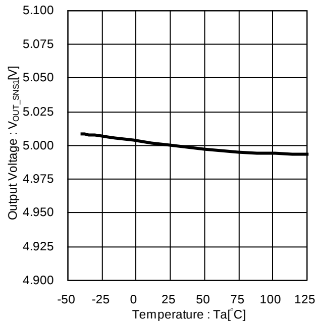
Figure 12. Output Voltage vs Temperature (BD9P255EFV-C)
