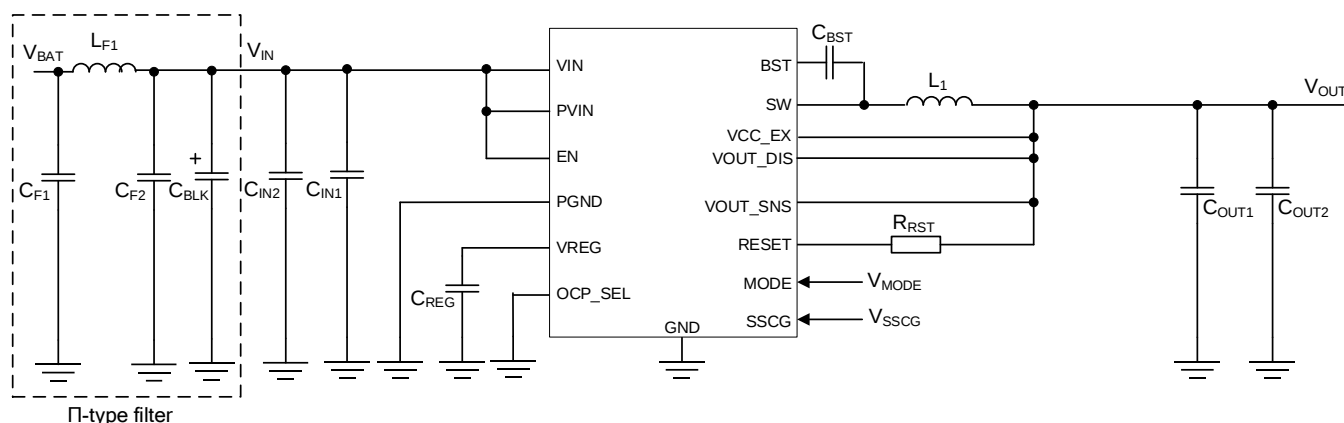
Figure 62. Reference Circuit 2
