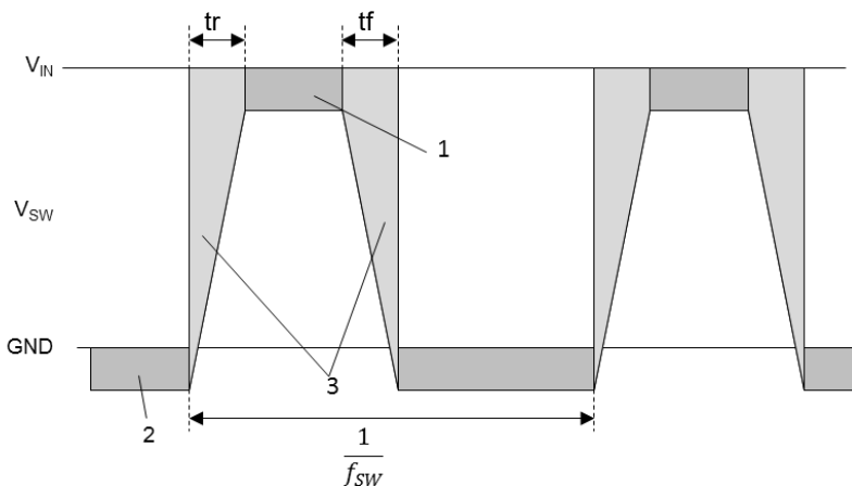
Figure 92. SW Waveform
