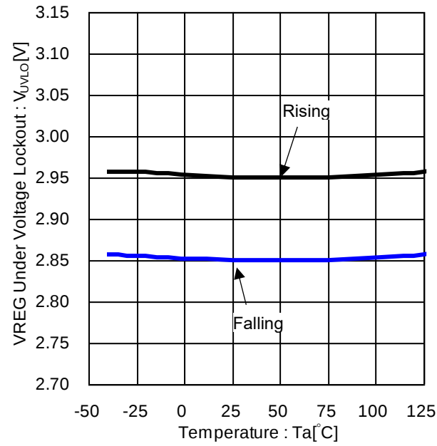
Figure 14. VREG Under Voltage Lockout vs Temperature
