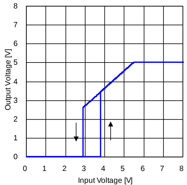
Figure 85. Output Voltage vs Input Voltage 2 ( R_{LOAD} = 2.5 \Omega )
