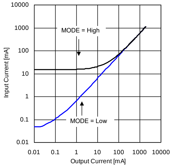
Figure 51. Input Current vs Output Current ( V_{IN} = 12\text{ V} )
