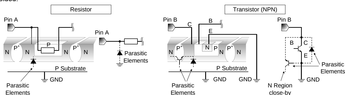
Figure 93. Example of Monolithic IC Structure
