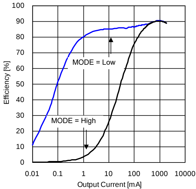
Figure 50. Efficiency vs Output Current ( V_{IN} = 12\text{ V} )
