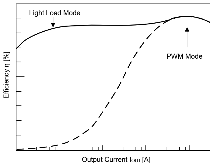
Figure 30. Efficiency (Light Load Mode, PWM Mode)
