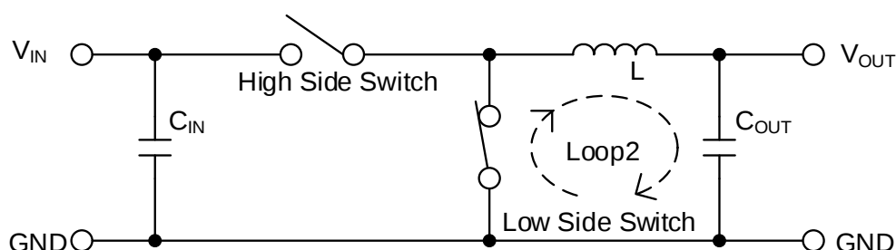
Figure 89 (b). Current Path when High Side Switch = OFF, Low Side Switch = ON
