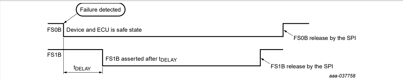
Figure 29. t_{DELAY} operation
