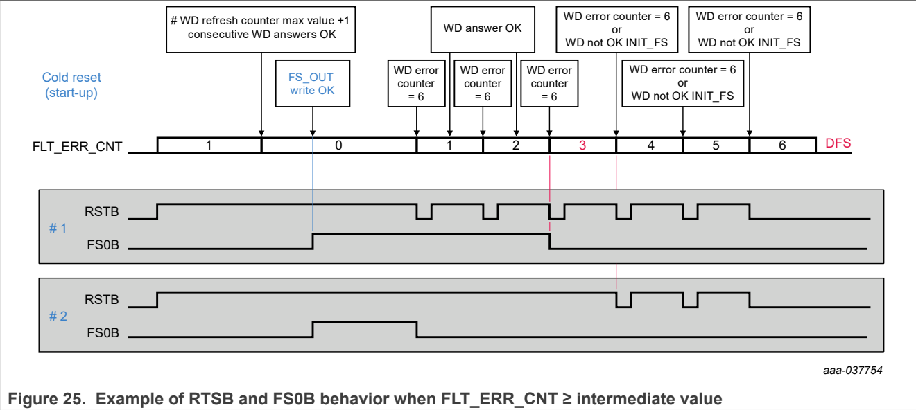
Figure 25. Example of RTSB and FS0B behavior when FLT_ERR_CNT ≥ intermediate value
