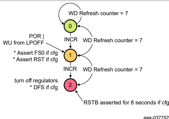
Figure 23. Fault error counter (FLT_ERR_FS = 1, WD_CNT_RFR = 6)
