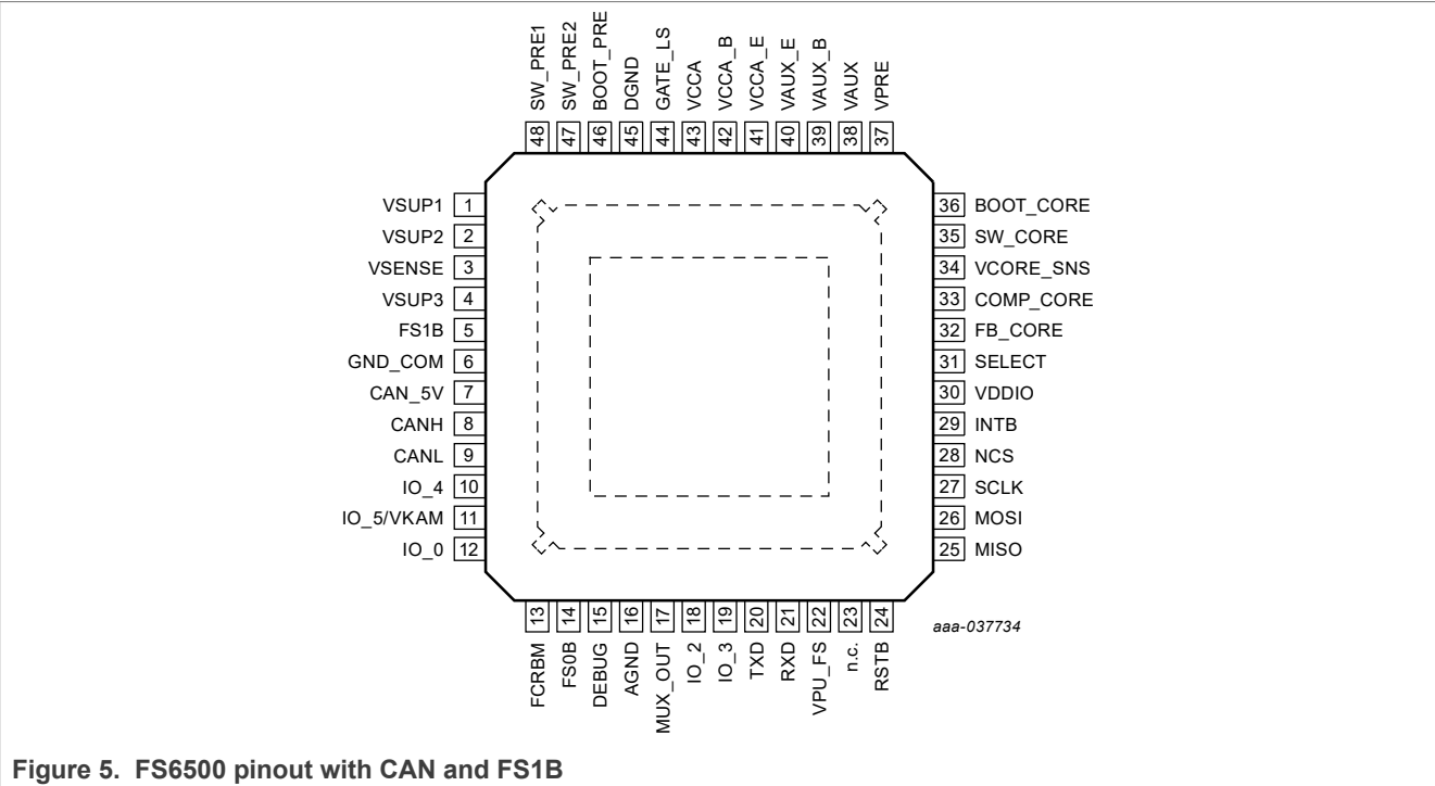
Figure 5. FS6500 pinout with CAN and FS1B
