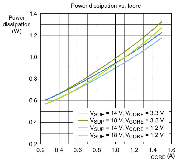
Figure 52. Power dissipation versus I_{CORE} , I_{CCA} , or I_{PRE}
