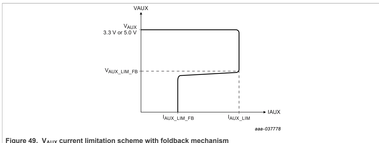
Figure 49. V_{AUX} current limitation scheme with foldback mechanism
