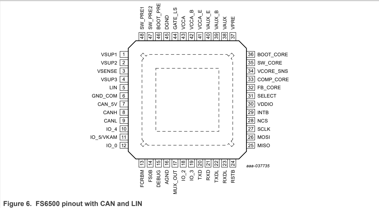
Figure 6. FS6500 pinout with CAN and LIN
