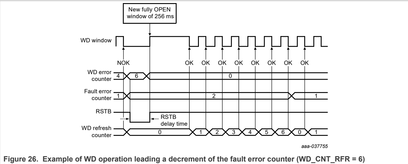
Figure 26. Example of WD operation leading a decrement of the fault error counter (WD_CNT_RFR = 6)
