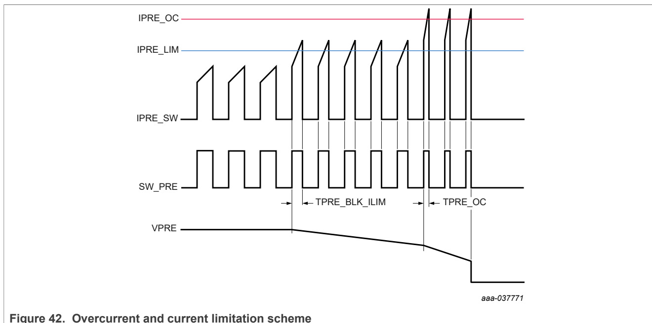
Figure 42. Overcurrent and current limitation scheme
