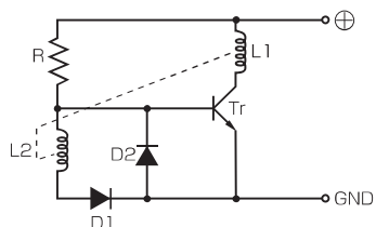
Fig. 2 Circuit diagram of type TMB
