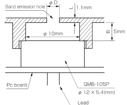
Fig. 6 Geometrical conditions
