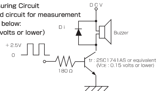
Fig. 2 Measuring Circuit
