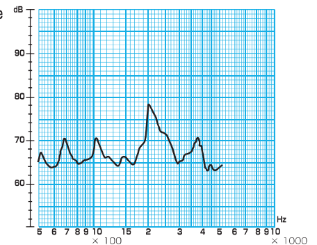
Fig. 5 Frequency response without additional resonator
