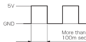
Fig. 3 Response time
