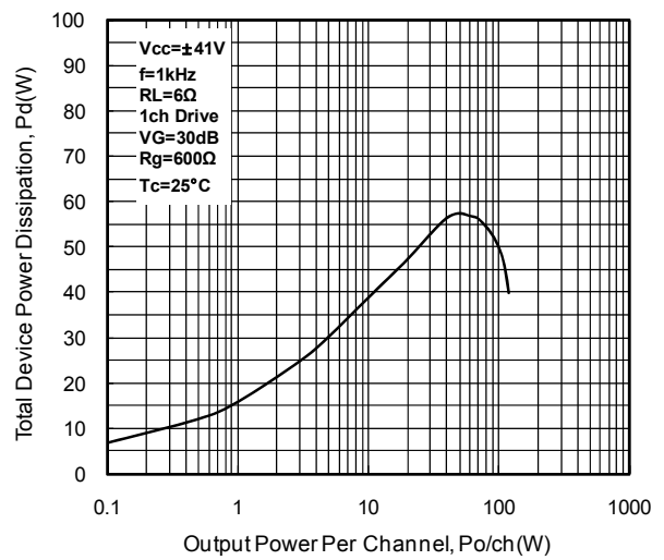
Pd-Po STK404-120N-E
