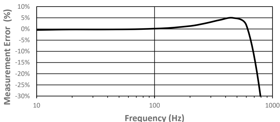
Typical Measurement Error vs. Frequency, Sinusoidal Input
