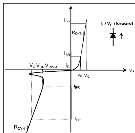
Fig. 8.1 Definitions of Electrical Characteristics
