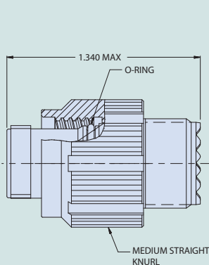
06- Plug
