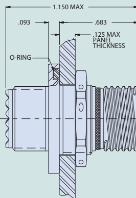
04- Jam Nut Receptacle with Wire Holes
