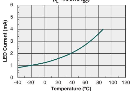
Typical I_F for Switch Dropout vs. Temperature ( I_L=100\text{mA}_{DC} )
