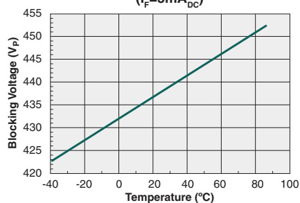
Typical Blocking Voltage vs. Temperature ( I_F=5\text{mA}_{DC} )
