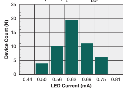
Typical I_F for Switch Operation (N=50, I_L=100\text{mA}_{DC} )
