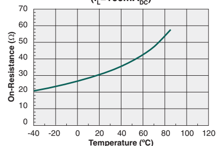
Typical On-Resistance vs. Temperature ( I_L=100\text{mA}_{DC} )
