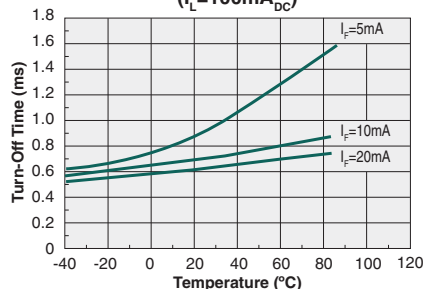
Typical Turn-Off Time vs. Temperature ( I_L=100\text{mA}_{DC} )
