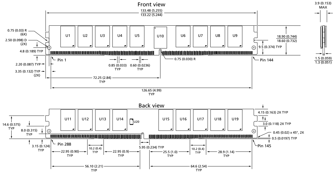
Figure 4: 288-Pin DDR4 VLP RDIMM (PCB 1714, 2463)
