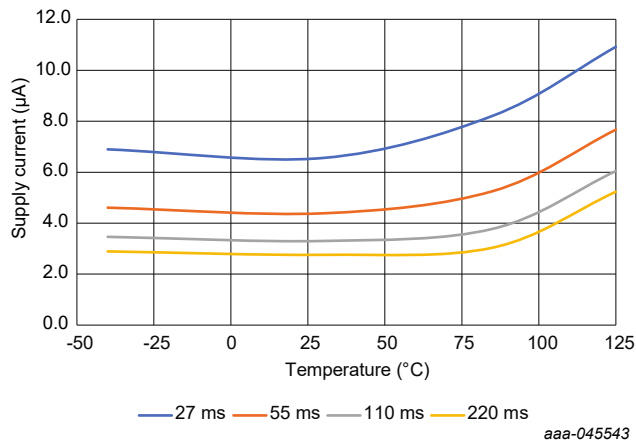
Figure 25. Supply current versus conversion time and temperature ( V_{CC} = 1.8\text{ V} , bus inactive)
