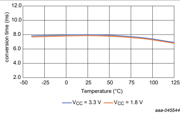
Figure 26. One-shot conversion time versus temperature
