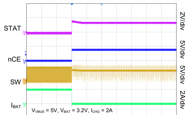
Charge Disable
