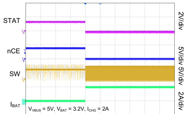
Charge Enable
