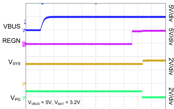
VBUS Power-Up with Charge Disable ( V_{BAT} = 3.2V )
