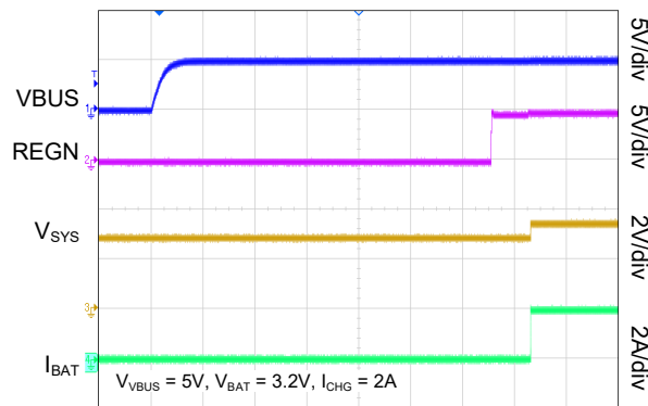
VBUS Power-Up with Charge Enable ( V_{BAT} = 3.2V )
