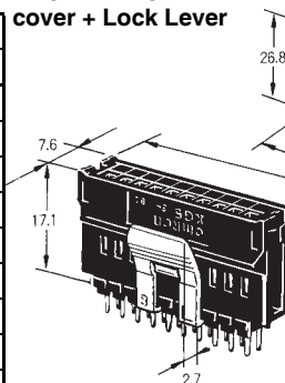
Original Plug + Semi-cover + Lock Lever
