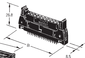
MIL Plug + Semi-cover
