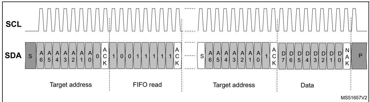
Figure 24. FIFO read
