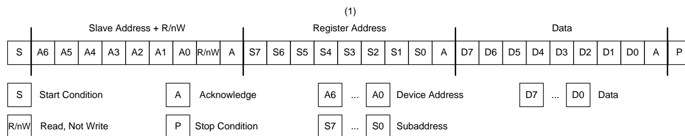
Figure 5-31. Subaddress in I 2 C Transmission
