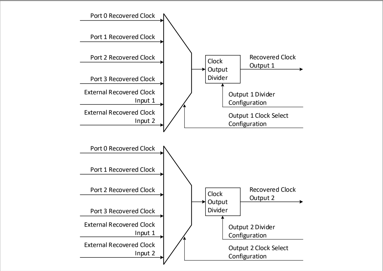
FIGURE 5-3: SYNCN RECOVERED CLOCK OUTPUTS
