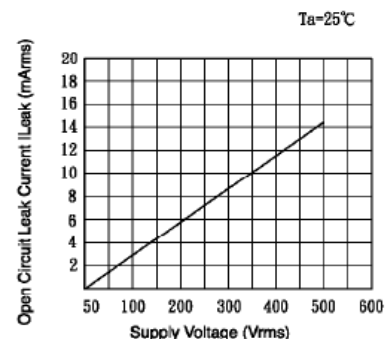
Fig.3 Open Circuit Leak Current vs. Supply Voltage
