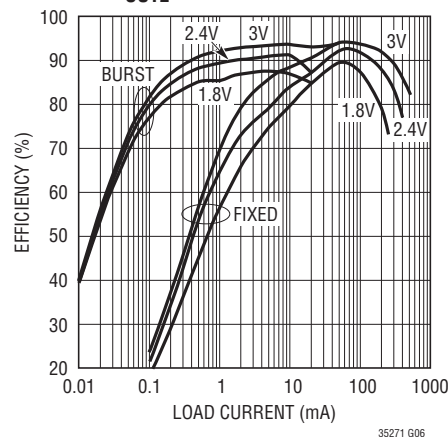
Efficiency vs Load Current and V_{IN} for V_{OUT2} = 3.3\text{V} at 2.2MHz
