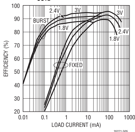
Efficiency vs Load Current and V_{IN} for V_{OUT2} = 3.3\text{V} at 1.2MHz
