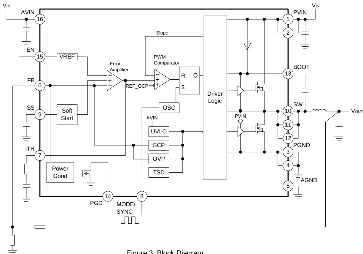
Figure 3. Block Diagram
