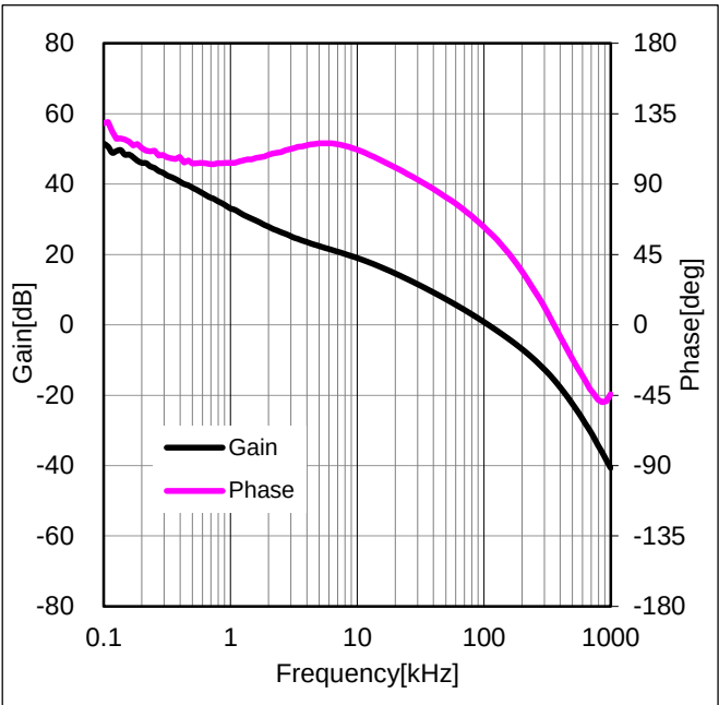
Figure 63. Frequency Characteristics ( I_{OUT}=2A )
