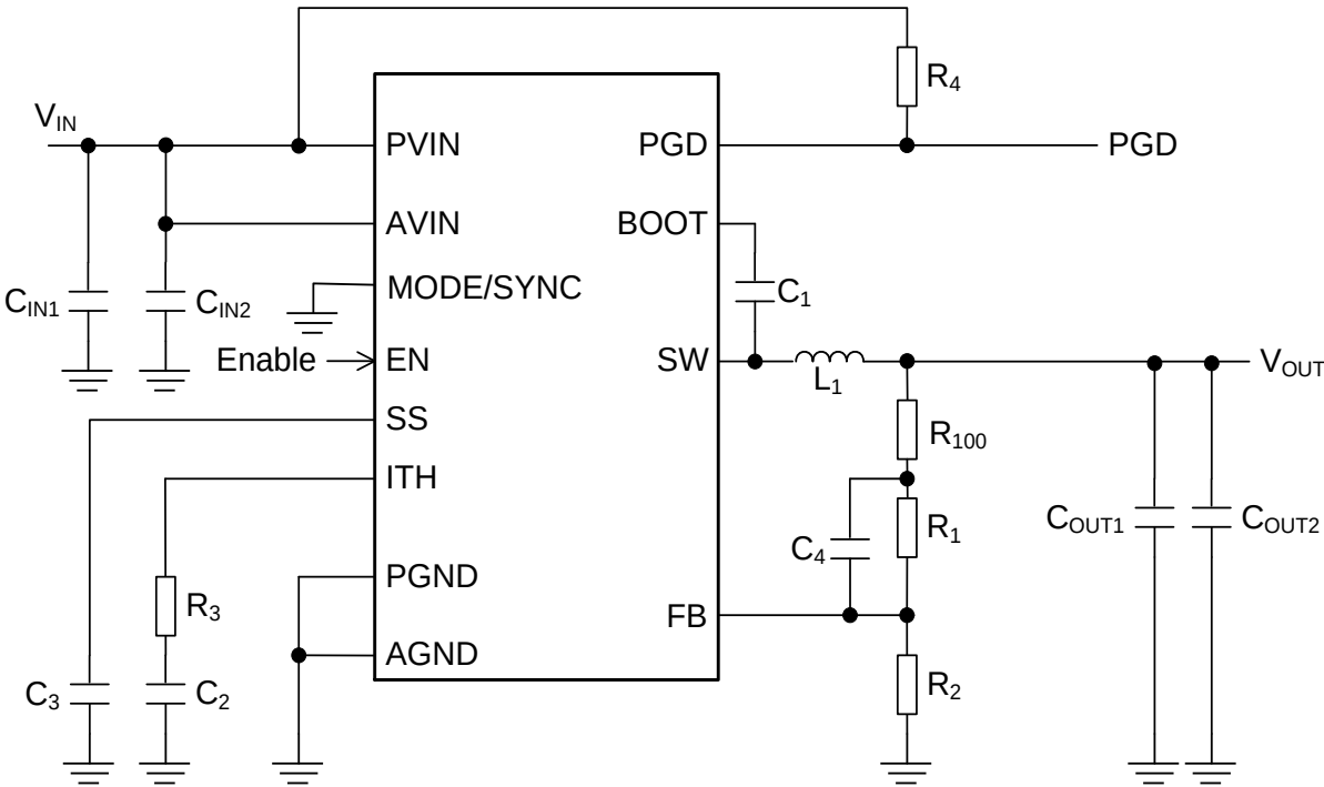
Figure 51. Reference Circuit 3
