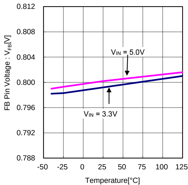
Figure 7. FB Pin Voltage vs Temperature
