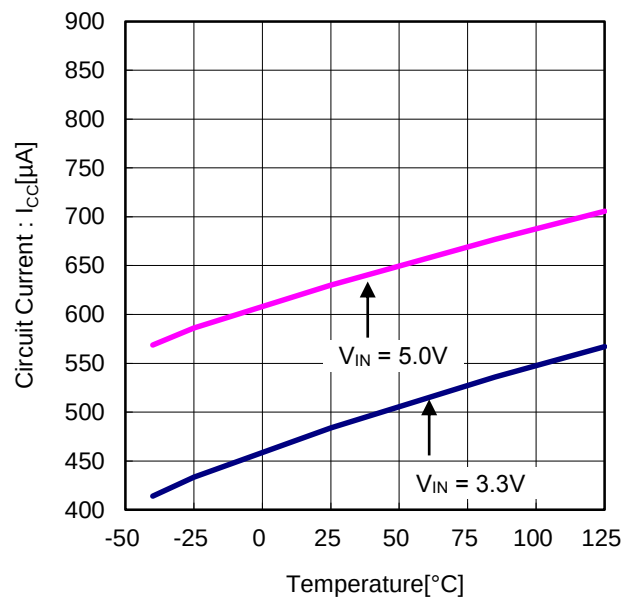
Figure 5. Circuit Current vs Temperature
