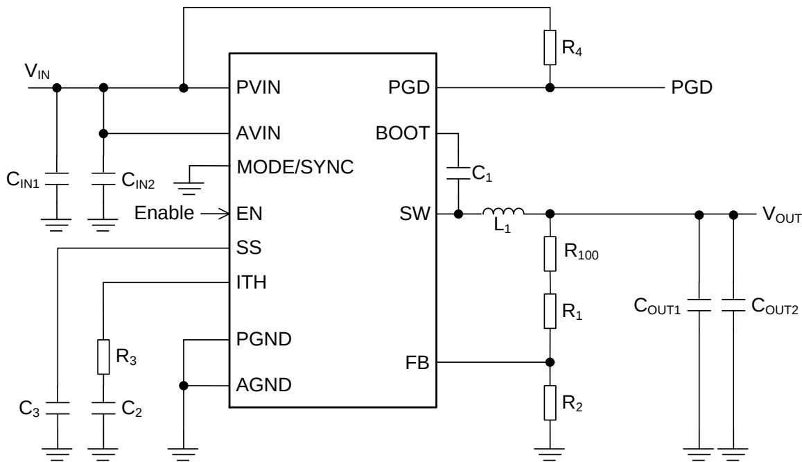
Figure 34. Typical Application
