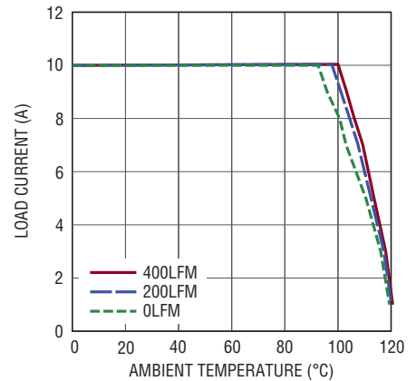
Figure 13. No Heat Sink with 3.3V IN to 2.5V OUT
