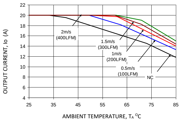
Figure 12. V_o = 5.0\text{ V}
