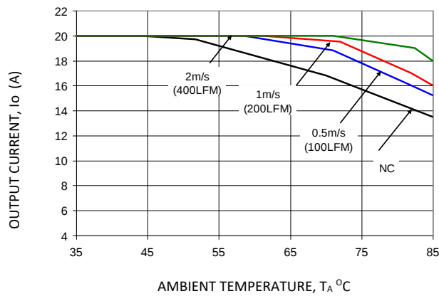
Figure 7. V_o = 0.69\text{ V}
