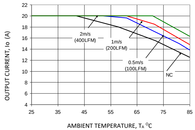
Figure 8. V_o = 1.2\text{ V}
