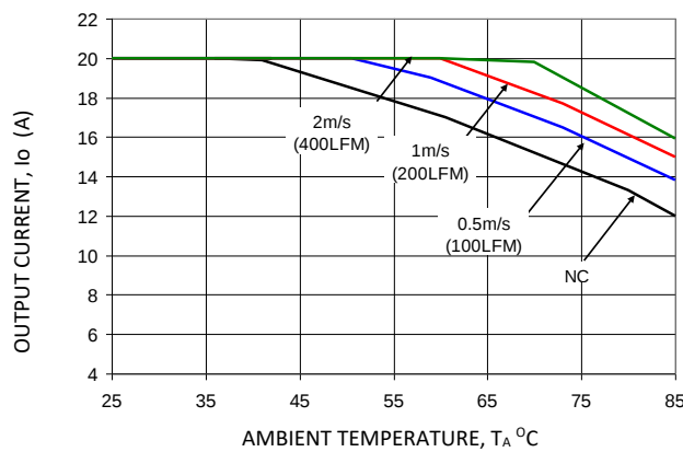
Figure 11. V_o = 3.3\text{ V}
