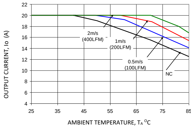
Figure 9. V_o = 1.8\text{ V}
