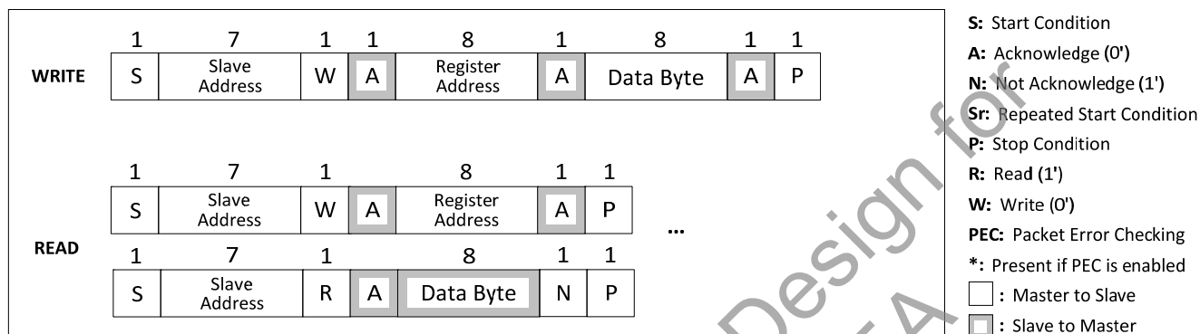
Figure 51: I2C Format
