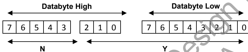
Figure 59: 11-bit Linear Data Format
