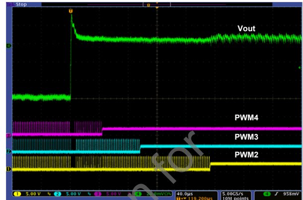
Figure 38: Phase Shed 4Φ→1Φ
