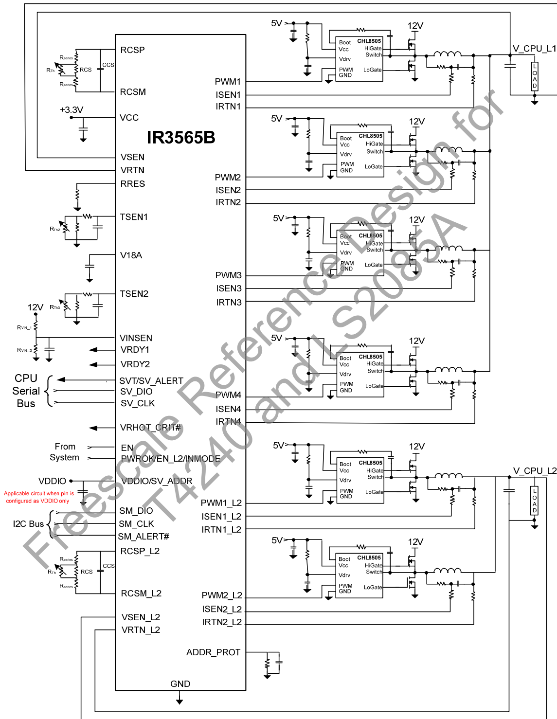
Figure 3: Dual-loop VR using IR3565B Controller and CHL8505 MOSFET Drivers in 4+2 Configuration
