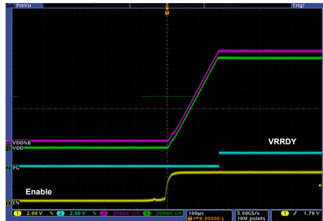
Figure 10: Enable-based Startup
