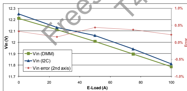
Figure 49: I2C Input Voltage Measurements
