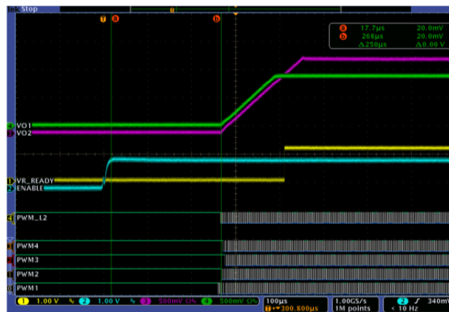
Figure 15: Loop 1 & Loop 2 start together with 0.25ms delay from Enable
