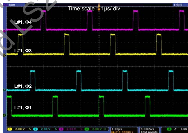
Figure 21: 4-phase PWM interleaved operation
