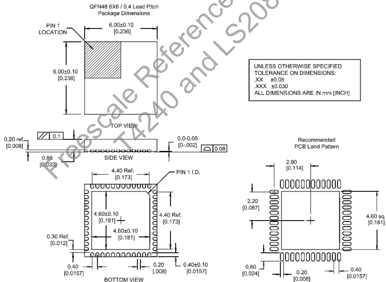
Figure 62: Package Dimensions
