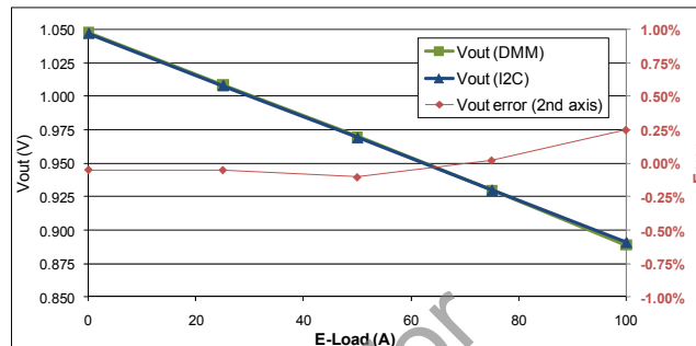
Figure 50: I2C Output Voltage Measurements
