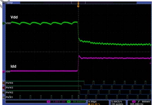
Figure 39: Phase Add 1Φ→4Φ
