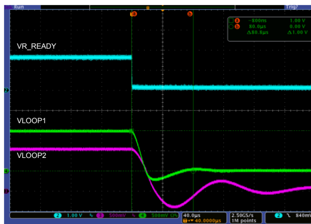
Figure 43: OVP - MOSFET latched on
