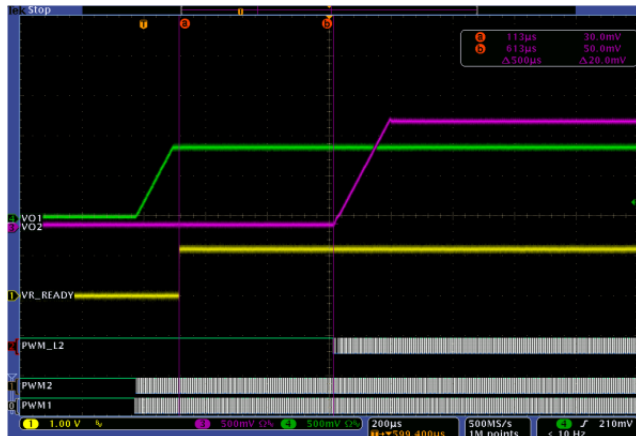
Figure 16: Loop 2 starts when Loop 1 VRRDY = high with 0.5ms delay between the loops
