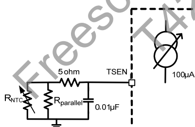
Figure 46: Temperature Sense NTC Network
