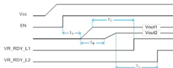
Figure 18: MPoL Startup
