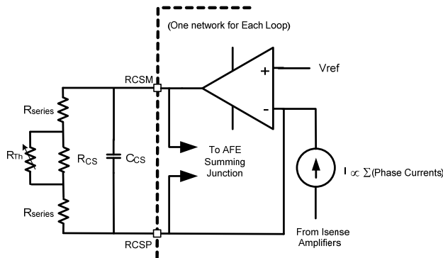
Figure 30: Load Line & Thermal Compensation
