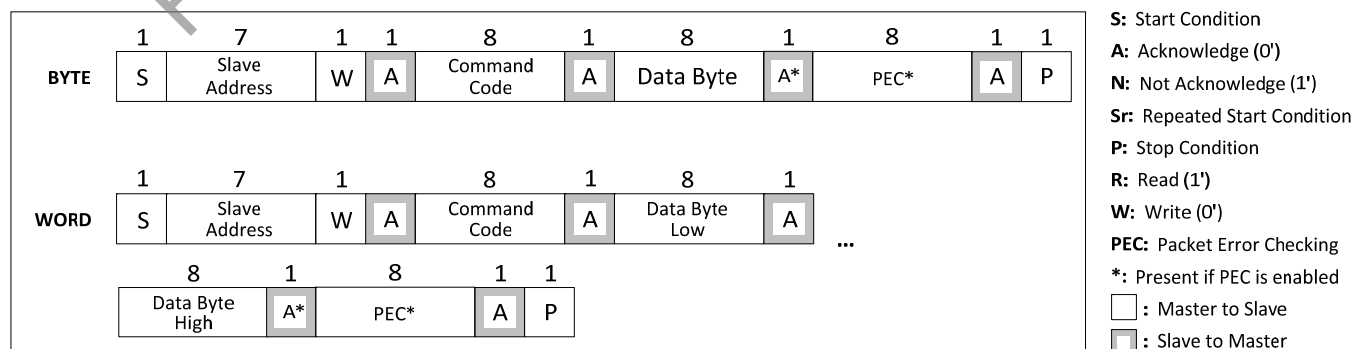
Figure 52: SMBus Write Byte/Word
