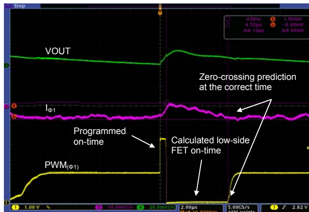
Figure 42: PS2 Active Diode Emulation Mode
