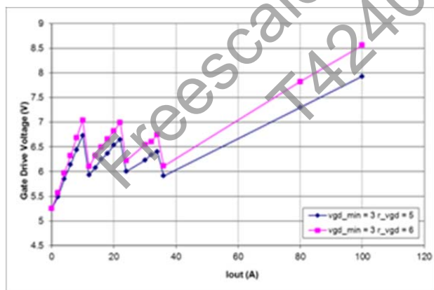
Figure 36: Variable Gate Drive Voltage versus Load Current
