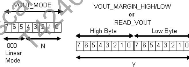
Figure 60: 16-bit Linear Data Format
