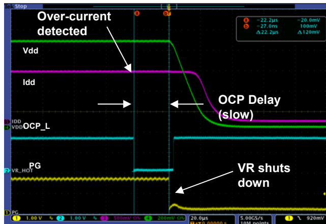
Figure 14: OCP_L (VR_HOT) assertion with OCP_TDC (Slow) threshold. OCP delay action (22µsec)
