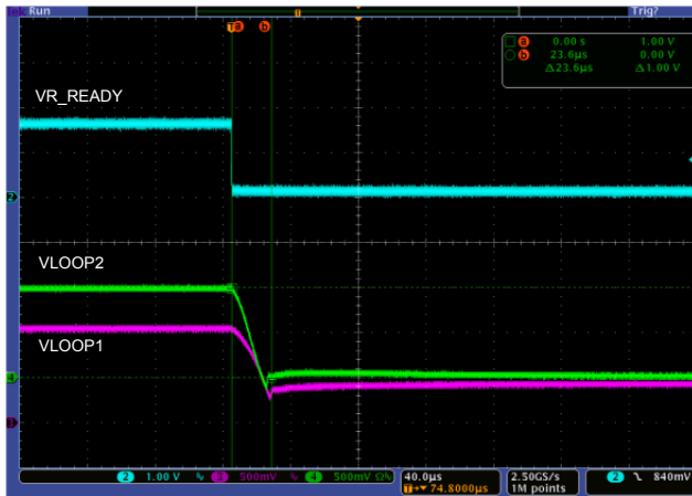
Figure 44: OVP - MOSFET released when output<0.5V
