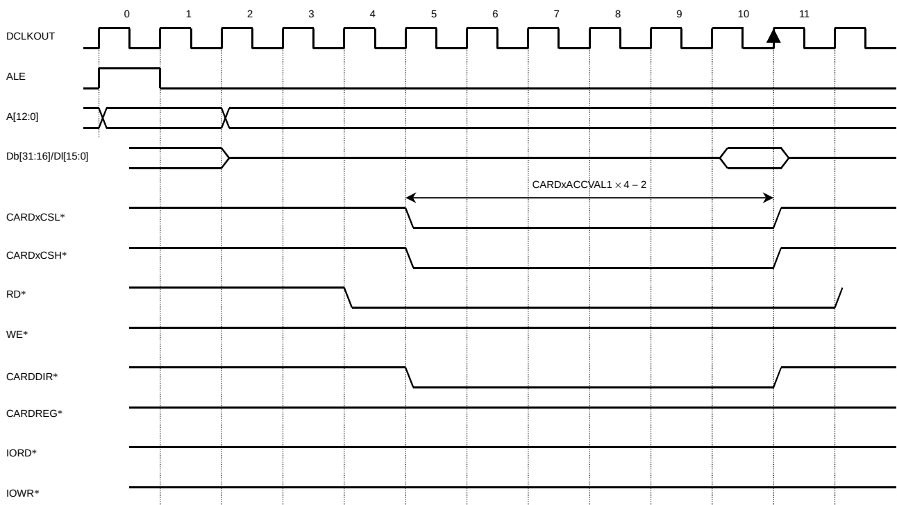
Figure B.21 16-bit CARD Device: Memory Access; Read Operation (2) (Half Word)
