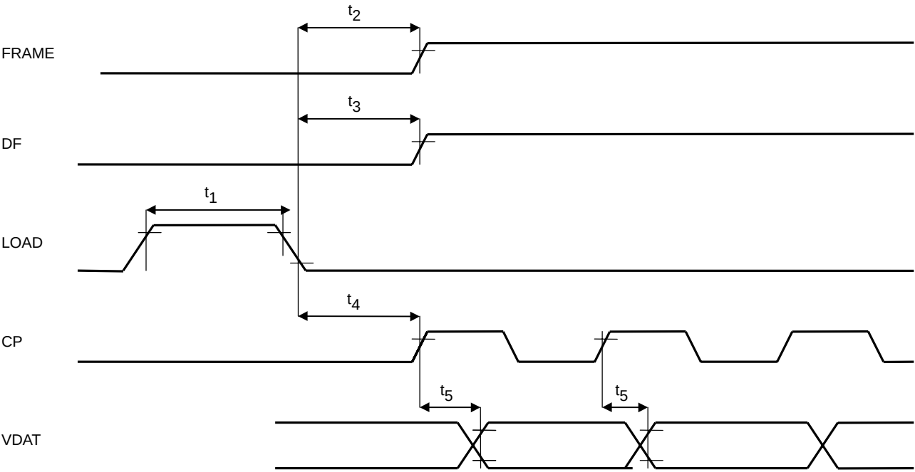
VIDEO Timing
