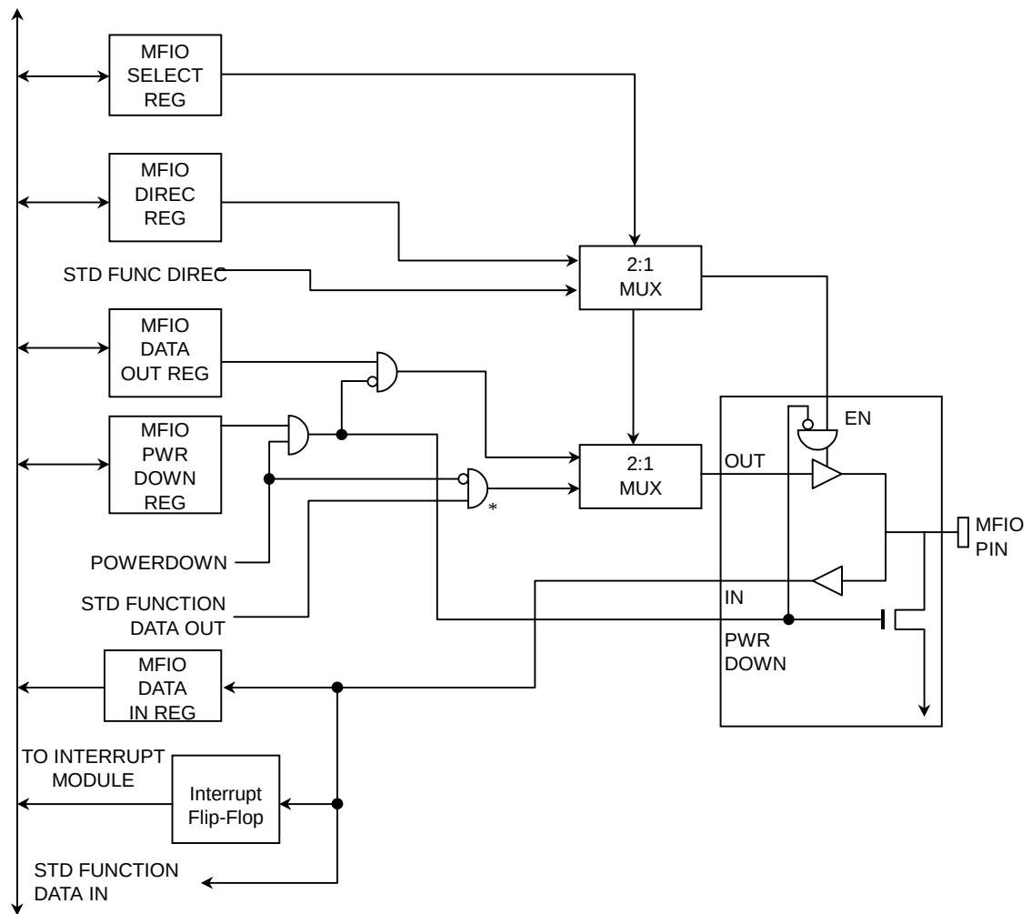
Figure 9.2.2 Multi-Function I/O Port Block Diagram
