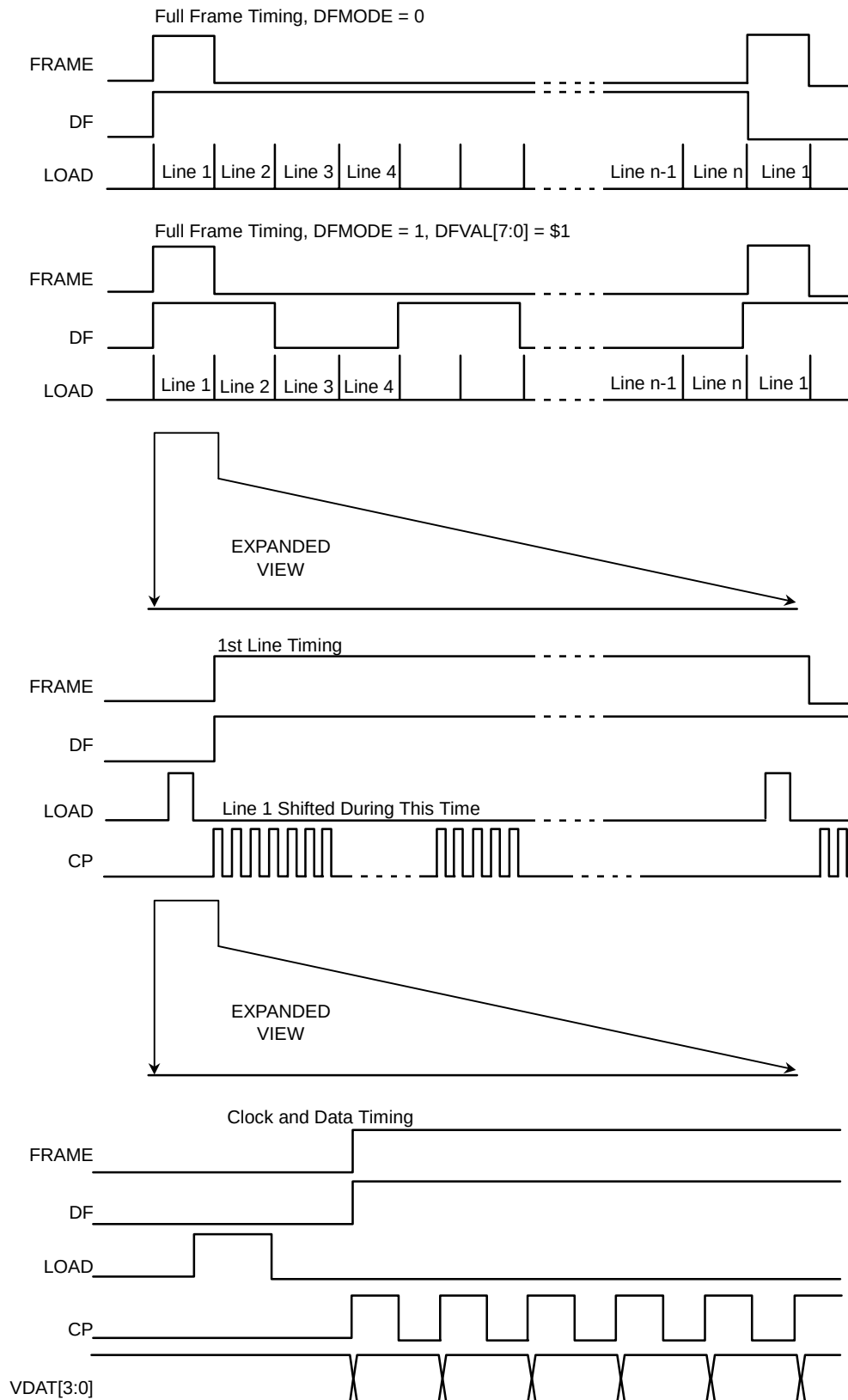
Figure 17.2.3 LCD Timing
