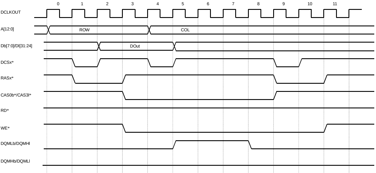
Figure B.61 8-bit SDRAM: Write Operation (1) (Byte)
