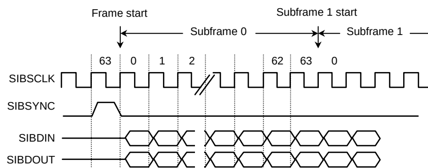
Figure 13.3.2 SIB Timing Relationships
