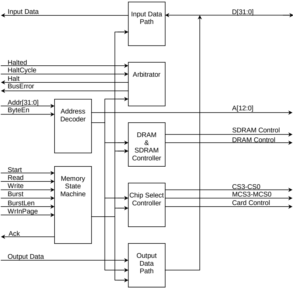
Figure 4.1.1 BIU Block Diagram
