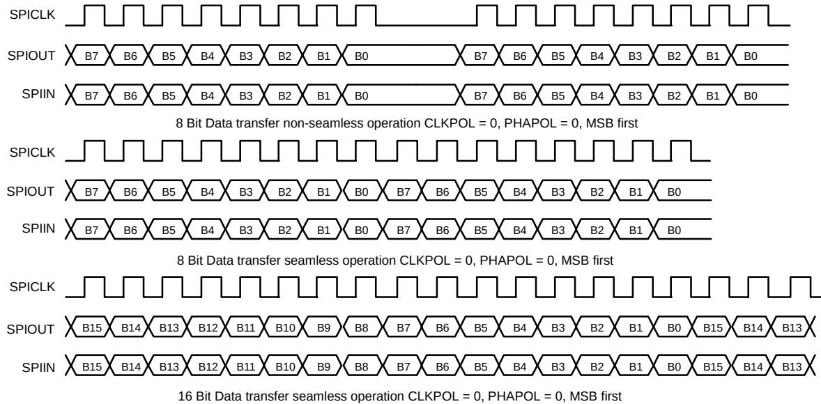
Figure 14.2.2 SPI Timing
