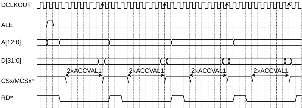
Figure 4.3.3 4-Word Burst Read 32-Bit Port
