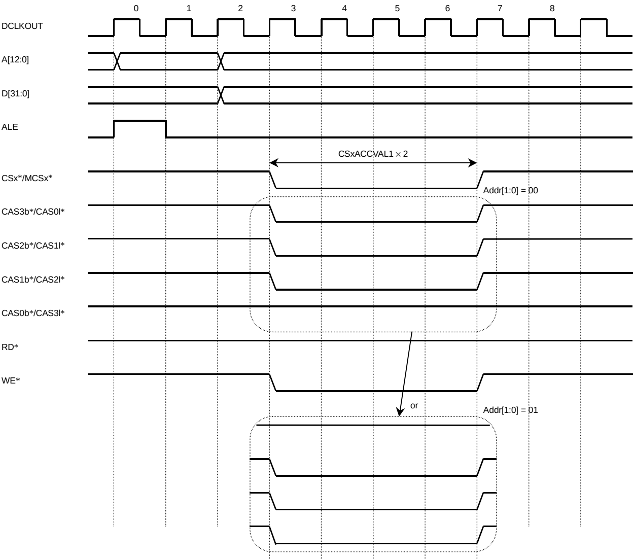
Figure B.12 32-bit Chip Select Device: Write Operation (3) (Triplebyte)
