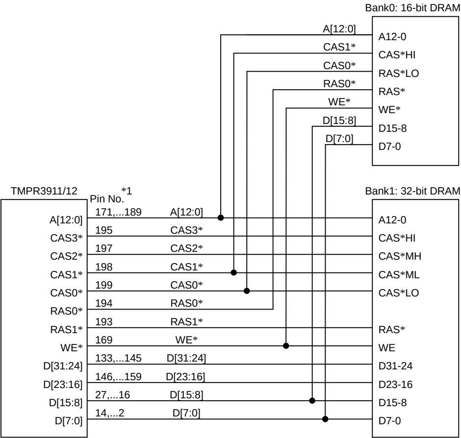
Figure 4.6.5 DRAM Memory Connection (Big Endian)*
