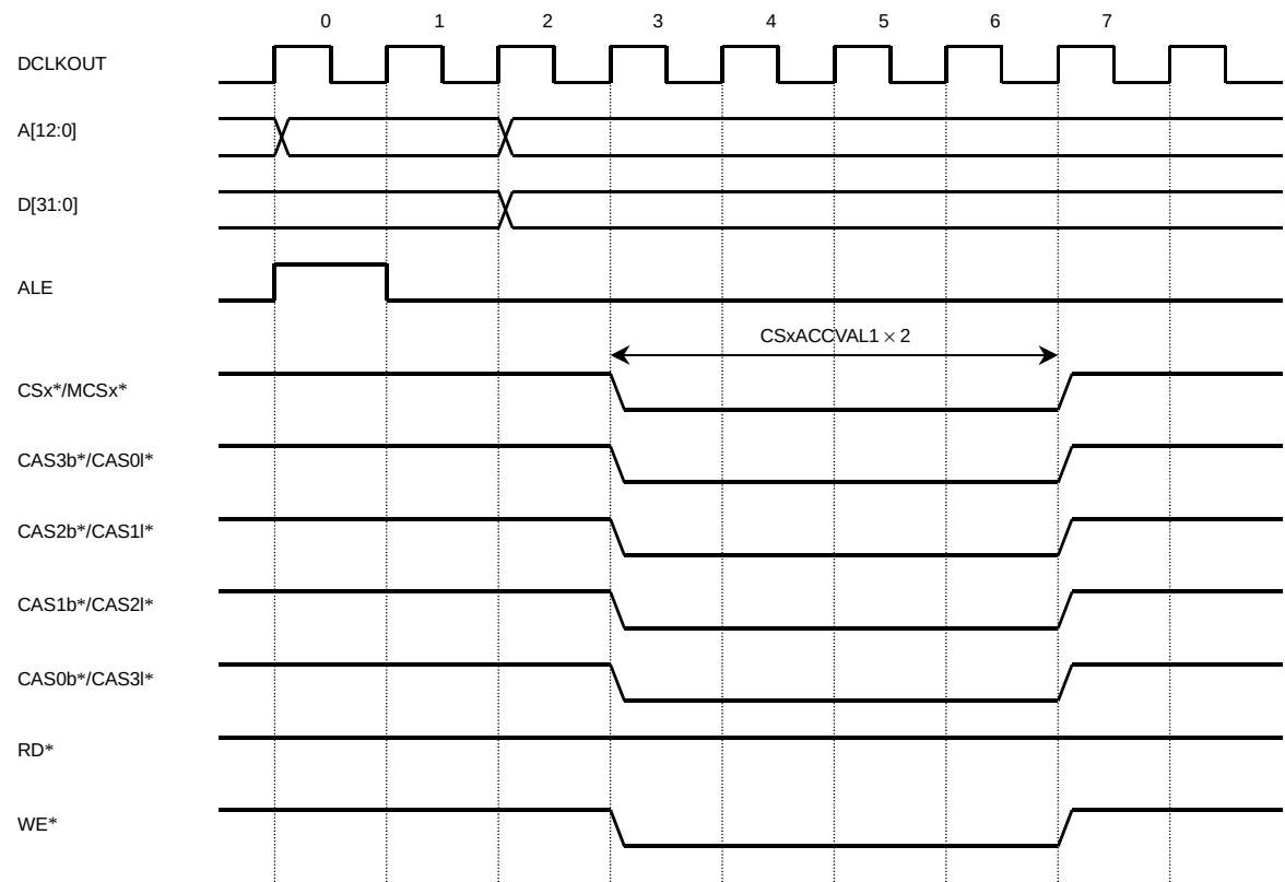
Figure B.13 32-bit Chip Select Device: Write Operation (4) (Word)
