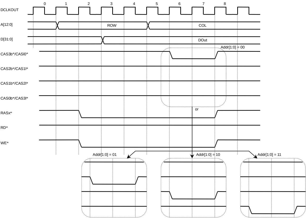
Figure B.51 32-bit DRAM: Write Operation (1) (Byte)
