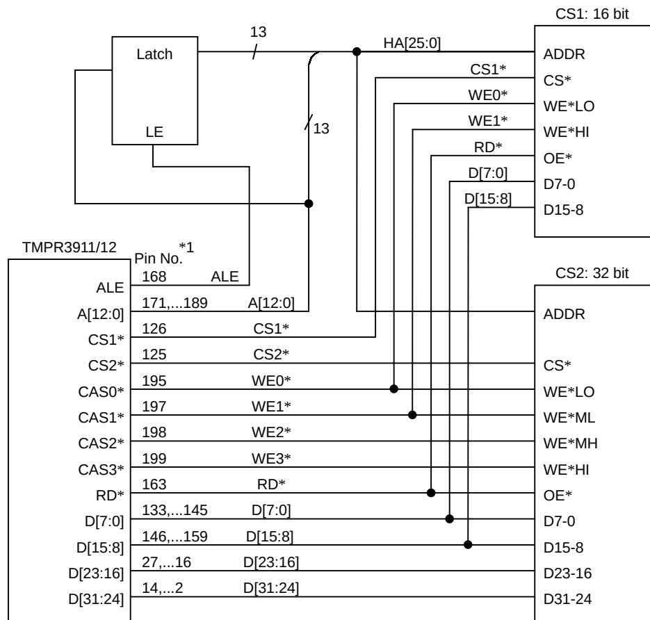
Figure 4.6.8 Chip Select Memory Connection (Little Endian)*
