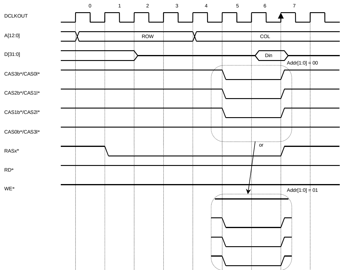
Figure B.58 32-bit DRAM: Read Operation (3) (Triplebyte)
