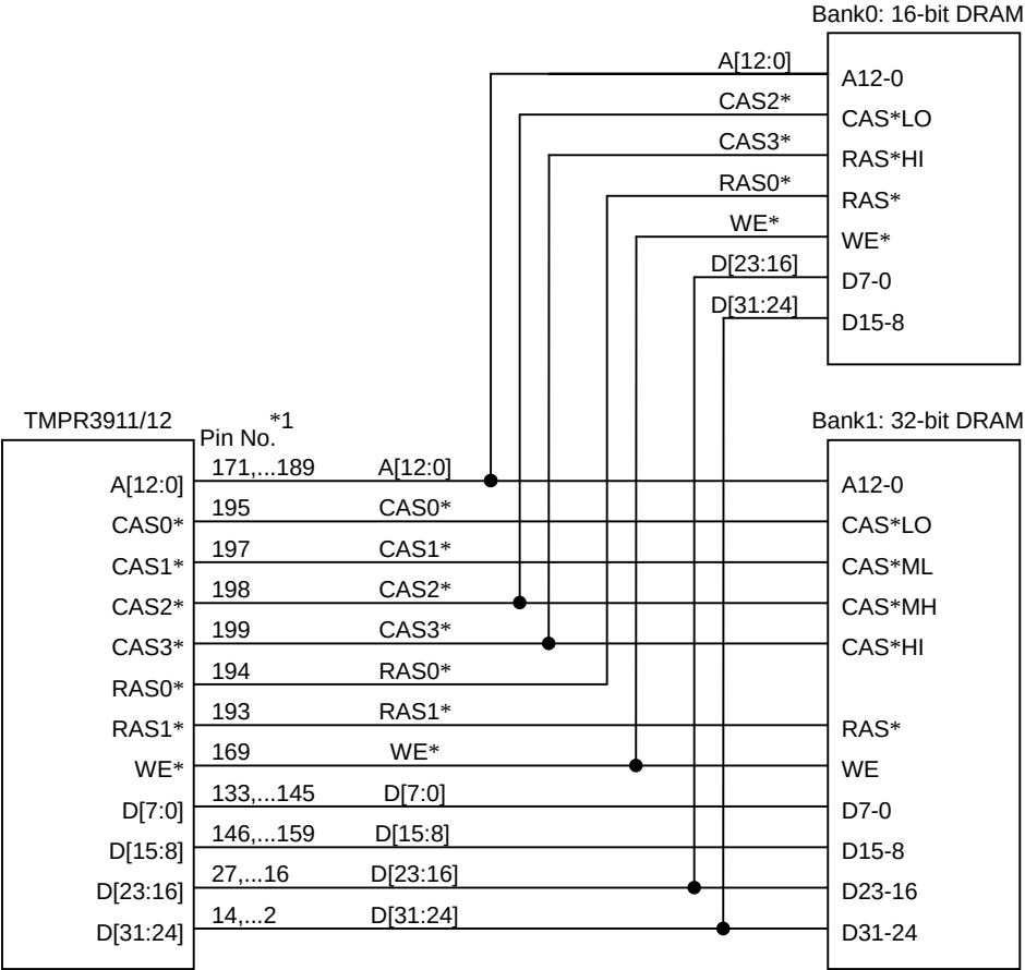
Figure 4.6.6 DRAM Memory Connection (Little Endian)*
