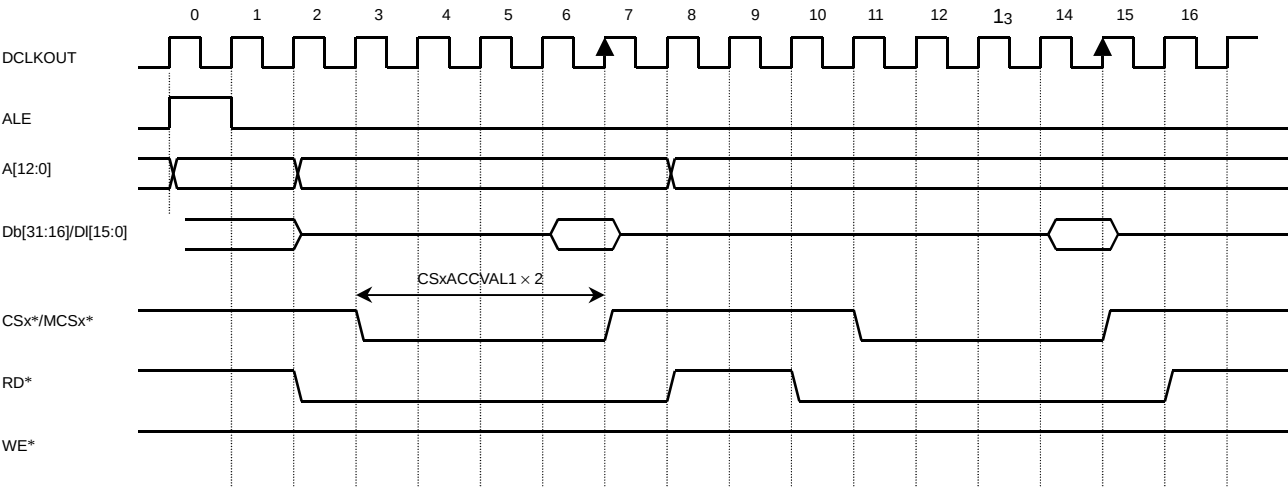
Figure B.8 16-bit Chip Select Device: Read Operation (4) (Word)
