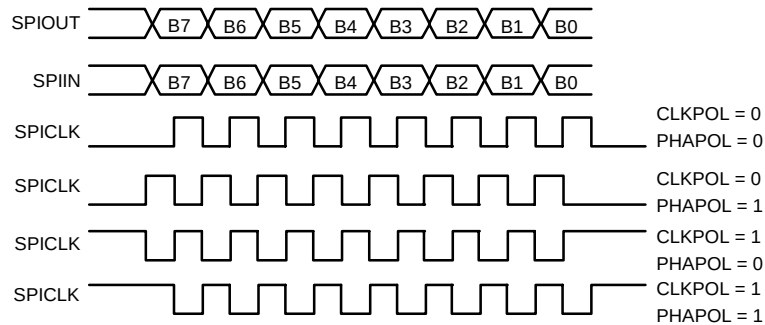
Figure 14.2.3 CLKPOL/PHAPOL Timing
