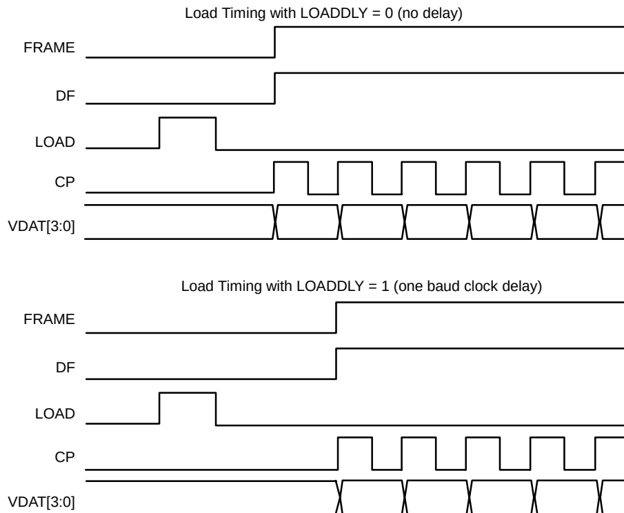
Figure 17.3.2 LOADDLY Timing
