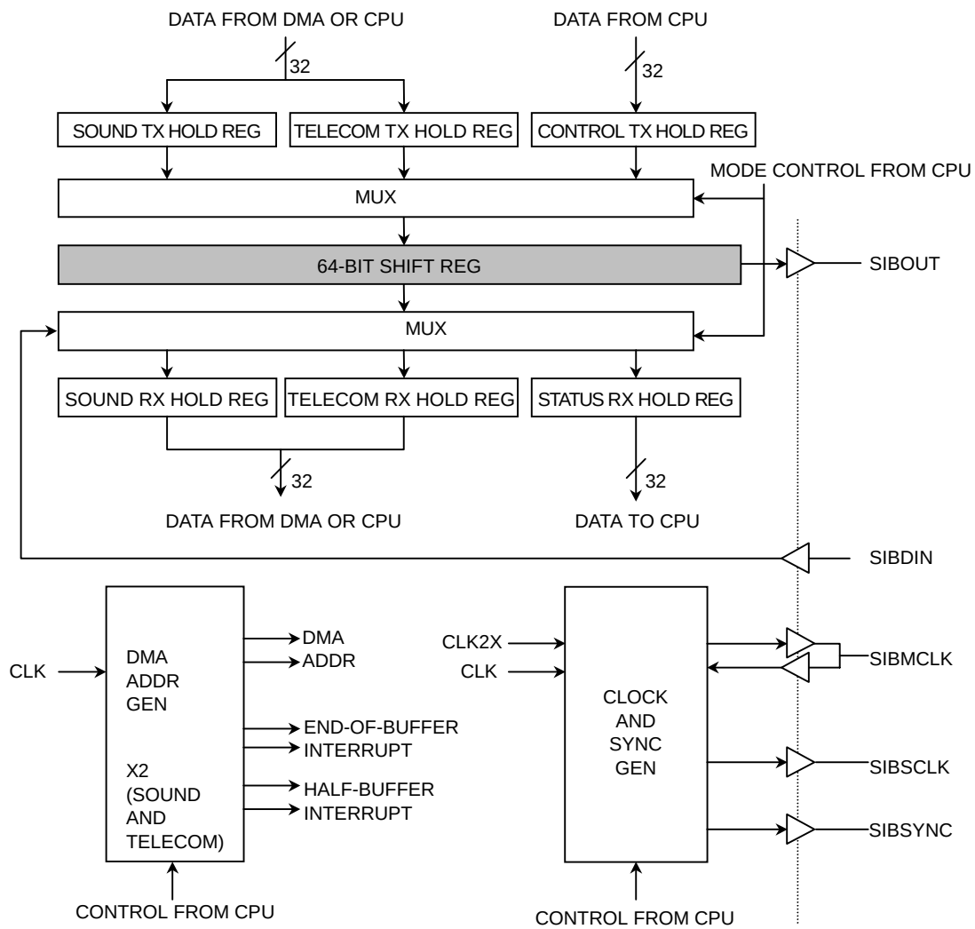
Figure 13.2.1 SIB Module Block Diagram
