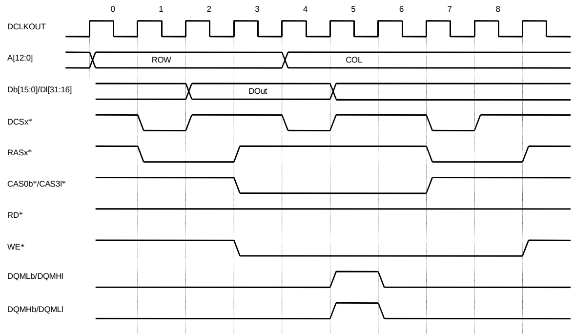
Figure B.69 16-bit SDRAM: Write Operation (2) (Halfword)
