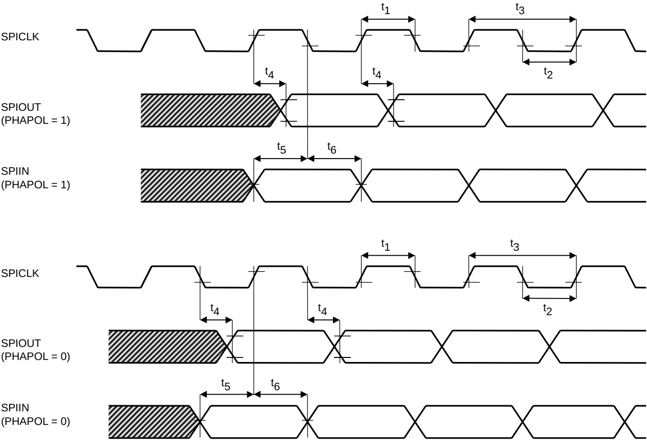
SPI Timing
