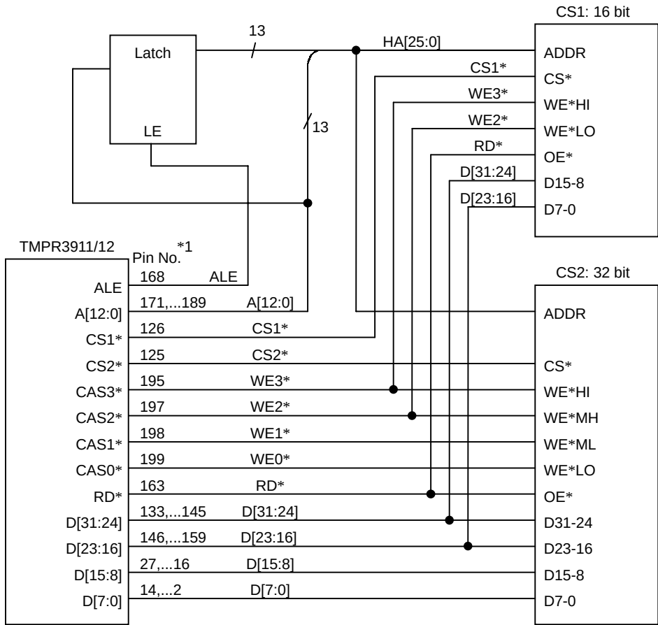
Figure 4.6.7 Chip Select Memory Connection (Big Endian)*
