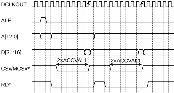
Figure 4.3.2 Word Read 16-Bit Port
