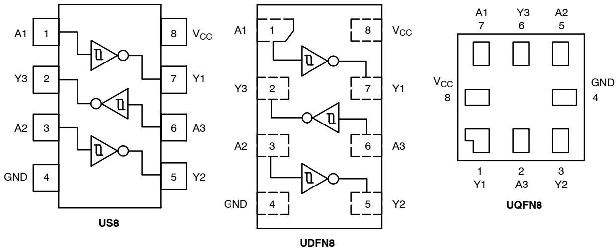
Figure 2. Pinout
