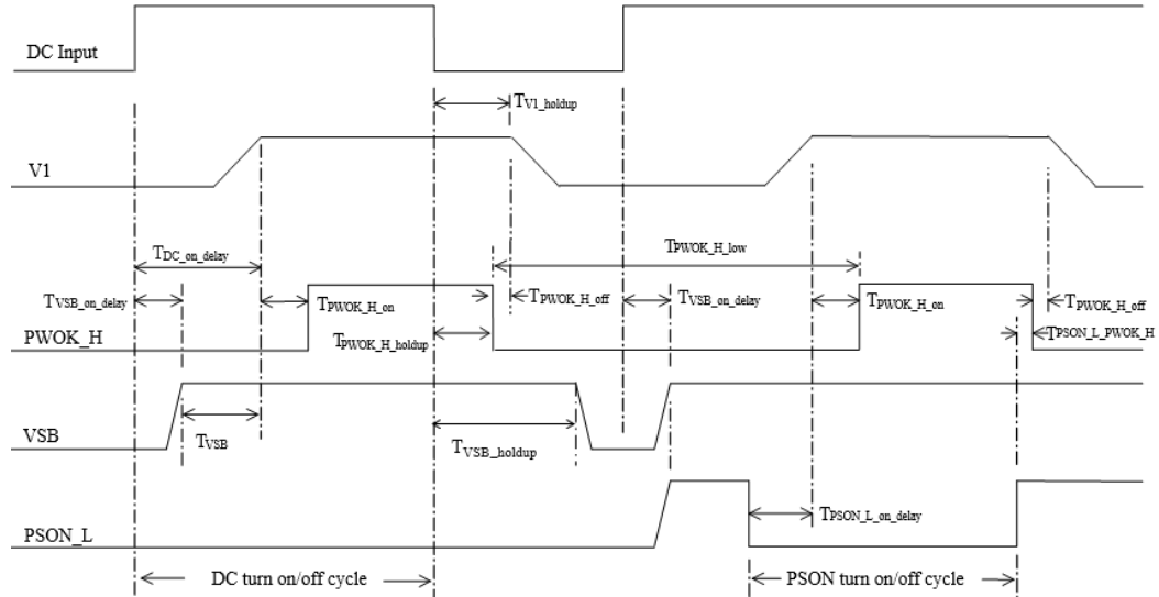
Figure 14. Timing Requirement
