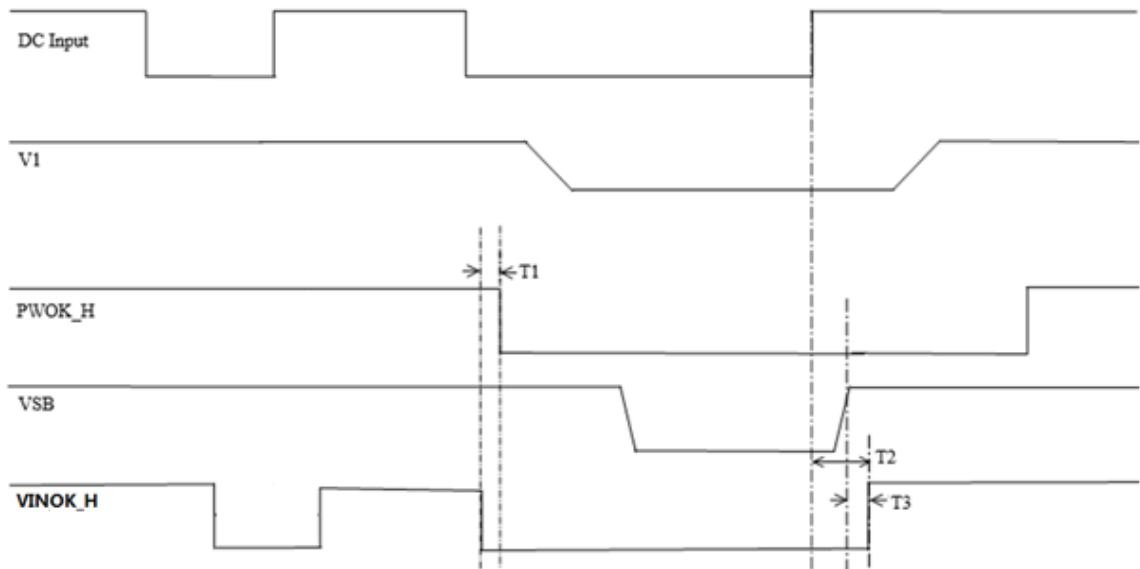
Figure 13. VINOK_H Timing
